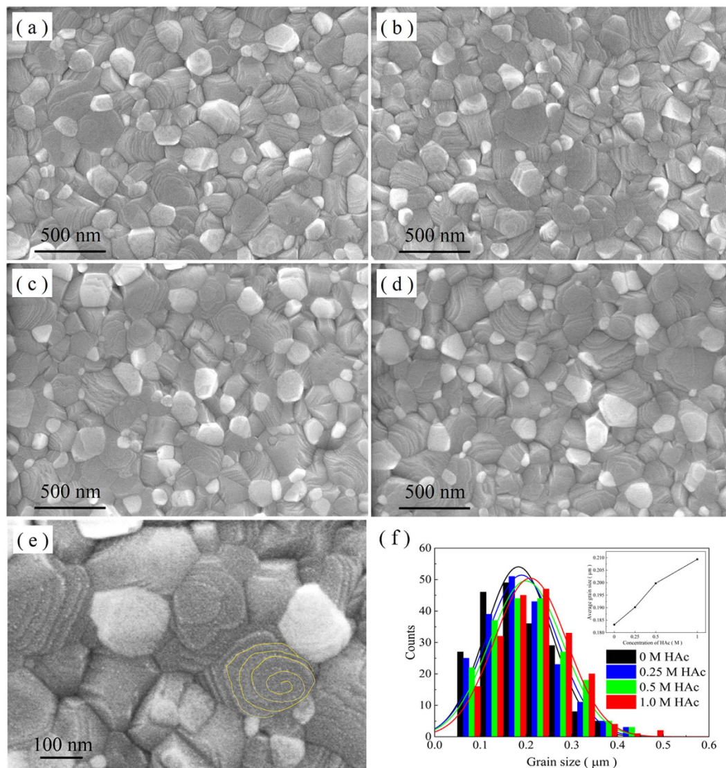
Figure 2. The morphology of films based on \text{PbAc}_2 by SEM. (a–d) The image of perovskite films deposited on a FTO/compact- \text{TiO}_2 substrate from the precursor solution containing different amounts of HAC, 0 M, 0.25 M, 0.5 M and 1.0 M, respectively. (e) SEM partial enlarged detail of (c) showing characteristic of spiral growth of the perovskite grains. (f) A histogram comparing the difference of perovskite grain size formed with different amounts of HAC, based on a set of data measured with 200 grains for each sample. The inset in (f) shows the change of average grain size with different amounts of HAC.
