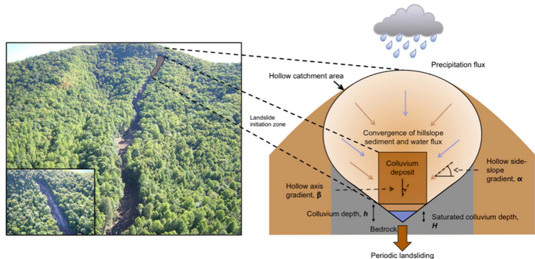
Figure 1. Shallow colluvium landslides in North Carolina. (Left) Photographs of the 2004 Peeks Creek landslide, triggered by intense precipitation during Hurricane Ivan (photos courtesy of Rick Wooten). (Right) Schematic diagram of colluvial hollow landslide recharge and triggering model.
