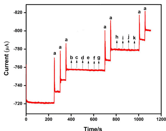
Figure 11. Amperometric i – t responses of H 2 O 2 reduction at Ag 2 MoO 4 modified RDGCE for the successive addition of 100 \mu\text{M} of H 2 O 2 (a), and 50-fold excess concentration of catechol (b), fructose (c), lactose (d), sucrose (e), glucose (f), hydroquinone (g), ascorbic acid (h), uric acid (i), dopamine (j) and epinephrine (k) in continuously stirred N 2 saturated 0.05 M PBS (pH 7). Applied potential: -0.5 V; Rotation rate: 1200 rpm.
