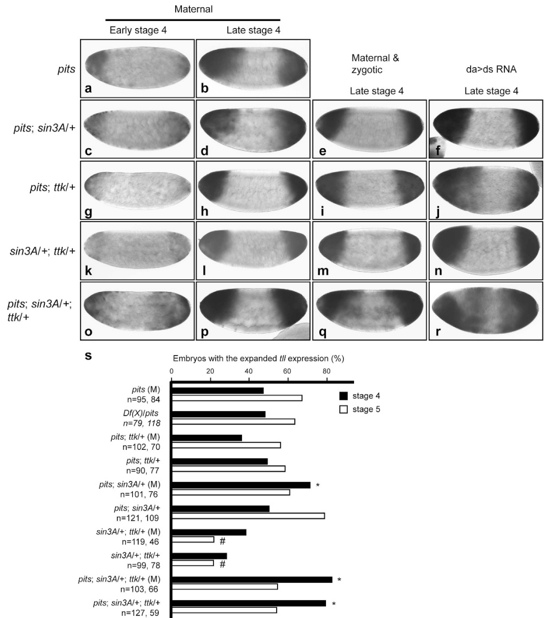
Figure 6. The genetic interactions of pits with sin3A and ttk are important for tll repression. To test the maternal effect of the gene activities, embryos from females pits 94 (a,b), pits 94 ; sin3A ex4 /+ (c,d), pits 94 ; ttk le11 /+ (g,h), sin3A ex4 /+; ttk le11 /+ (k,l) and pits 94 ; sin3A ex4 /+; ttk le11 (o,p) crossed with w 1118 males were collected to determine tll expression patterns. To test the maternal and zygotic effect of the genes' activities, females and males that had the same genotypes, as shown at the left, were mated (e,i,m,q). Due to undetectable GFP protein expressed by the ubi-GFP transgene in the balancer chromosome in early embryonic stages, genotypes of embryos homozygous for sin3A or ttk could not be determined. Therefore, RNAi was used. Females carrying the da-GAL4 transgene were mated with RNAi lines to knock down at least two gene activities simultaneously (f,j,n,r). The tll expression patterns in the embryos were revealed by in situ hybridization with digoxigenin-labeled antisense tll RNA. Embryos are arranged in a sagittal view, with the anterior towards the left. (s) A bar graph presents percentages of embryos with expanded tll expression patterns. "M" in brackets represents embryos only with reduced maternal gene activities. Percentage indicates proportion of embryos with expanded tll expression patterns over the total number of stage-4 (solid bars) or stage-5 (open bars) embryos. The left and right numbers beneath each genotype are the total numbers of stage-4 and stage-5 embryos. Df(X) represents Df(X)BSC624 . Fisher's exact test was used to determine statistical significance of proportion of embryos with the expanded tll expression from pits (M) mothers or Df(X)/pits crossed with pits males against those with further reduction of one or two more gene activities (*: increase, #: decrease, p < 0.001 ).
