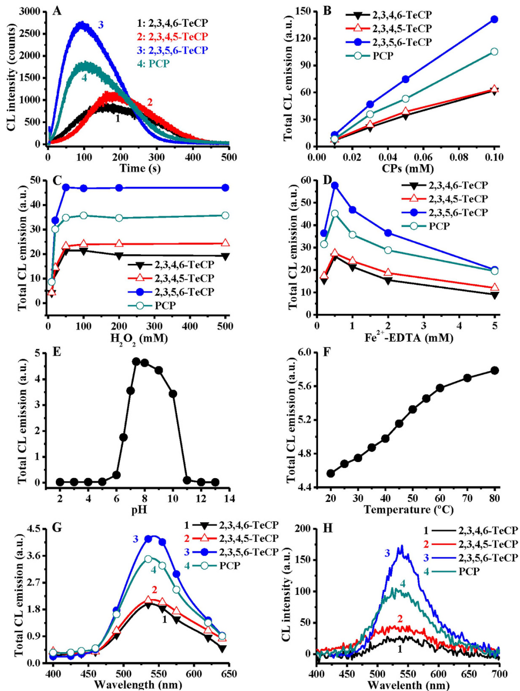
Figure 1. The CL emission could be produced during the degradation of TeCPs and PCP by Fenton system. (A) CL could be produced by TeCPs and PCP/Fenton system. TeCPs and PCP, 0.03 mM; \text{H}_2\text{O}_2 , 100 mM; \text{Fe}^{2+} -EDTA, 1 mM. (B–D) The dose-dependent effects of chlorophenols, \text{H}_2\text{O}_2 and \text{Fe}^{2+} -EDTA on CL production by chlorophenols/Fenton. TeCPs and PCP, 0.01–0.1 mM; \text{H}_2\text{O}_2 , 10–500 mM; \text{Fe}^{2+} -EDTA, 0.2–5 mM. (E,F) The effect of pH and temperature on CL production by 2,3,5,6-TeCP/Fenton. 2,3,5,6-TeCP, 0.03 mM; \text{H}_2\text{O}_2 , 100 mM; \text{Fe}^{2+} -EDTA, 1 mM. (G) The CL emission spectra measured by static-injection ultraweak CL analysis. TeCPs and PCP, 0.03 mM; \text{H}_2\text{O}_2 , 100 mM; \text{Fe}^{2+} -EDTA, 1 mM. (H) The CL emission spectra measured by spectrofluorometry. TeCPs and PCP, 2 mM; \text{H}_2\text{O}_2 , 1000 mM; \text{Fe}^{2+} -EDTA, 5 mM. All reactions were carried out in chelex-pretreated phosphate buffer (0.1 M, pH 7.4).
