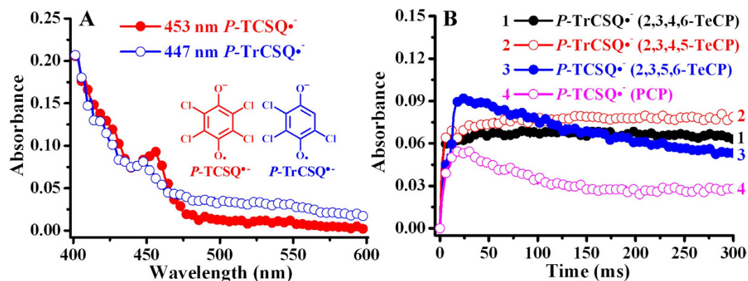
Figure 5. Transient P\text{-CSQs}^{\bullet-} production by TeCPs and PCP/Fenton system under the same experimental conditions for CL generation. (A) Transient absorption spectra of P\text{-CSQs}^{\bullet-} . (B) The kinetics of P\text{-TCSQ}^{\bullet-} formation at 453 nm and P\text{-TrCSQ}^{\bullet-} at 447 nm. TeCPs and PCP, 0.5 mM; \text{H}_2\text{O}_2 , 100 mM; \text{Fe}^{2+}\text{-EDTA} , 1 mM. All reactions were carried out in chelex-pretreated phosphate buffer (0.1 M, pH 7.4) at 25 °C.
