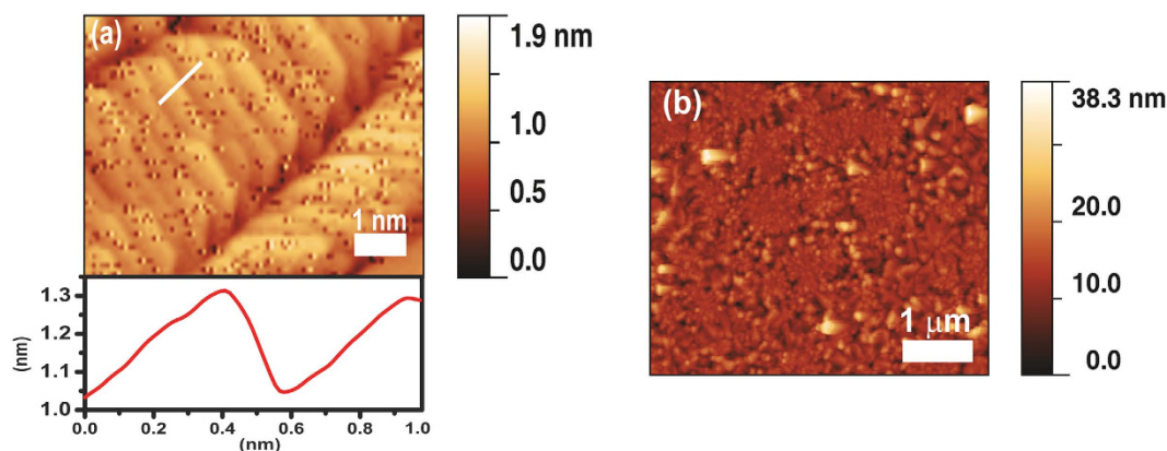
Figure 7. Topographic AFM images of the annealed films at 800\text{ }^\circ\text{C} : (a) Pure \text{TiO}_2 , with height profile of the atomic terraces and (b) 0.16\text{Ag-TiO}_2 .
