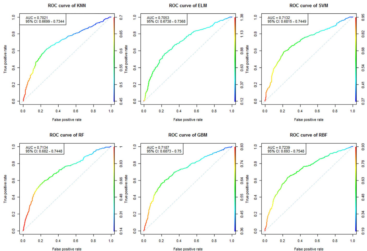
Figure 3. The ROC curve of six best benchmarked methods on the Psoriasis GWAS dataset of independent ADO group using selected best number of SNPs.
