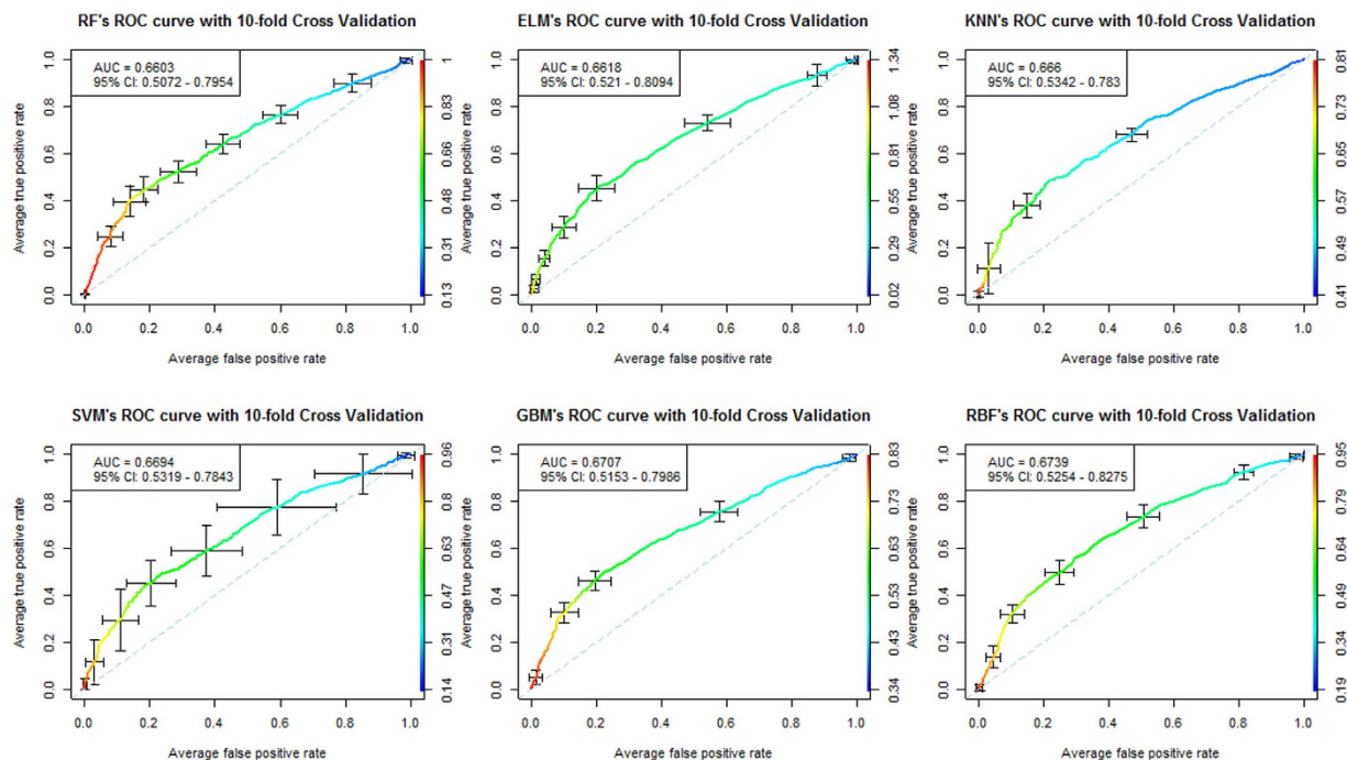
Figure 4. The average of ten-fold's cross-validation ROC curve of six best benchmarked methods on the Psoriasis GWAS dataset of GRU group using selected best number of SNPs.
