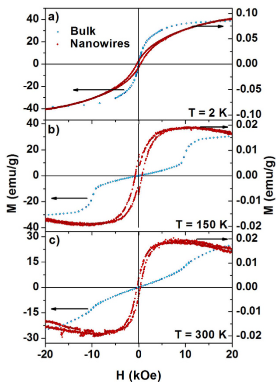
Figure 5. Field-dependent magnetization curves for \text{Fe}_3\text{Ga}_4 bulk (blue symbols, left axis) and nanowire array (red symbols, right axis): (a) 2 K (b) 150 K (c) 300 K.
