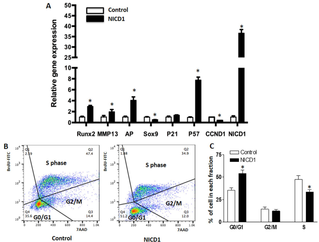
Figure 1. Notch activation promotes chondrocyte differentiation in ATDC5 cells by enhancing cell cycle exit. ATDC5 cells were transfected with NICD1 plasmids for 48 hours. Cells were then harvested for total RNA isolation and RT-PCR analysis. (A) Notch activation by NICD1 significantly increased NICD1, Runx2, MMP13, AP, and P57 gene expression and decreased Sox9 and Cyclin D1 (CcnD1) gene expression in culture. (B) Represented figure for cell cycle analysis. Cell population in S phase was largely reduced, and G0/G1 phase cell population was significantly increased at 48 hours post NICD1 transfection when compared to control cells. The cell cycle status was determined based on BrdU incorporation and staining with the DNA dye 7-AAD, and distribution in percentages are labeled in each dot plot. (C) Quantization of cell population in G0/G1, G2/M and S phase versus total cell population. PCR data are means \pm SD of three independent experiments performed in duplicate and the control gene expression level was set at 1. (* p < 0.05 compared with control at same time point).
