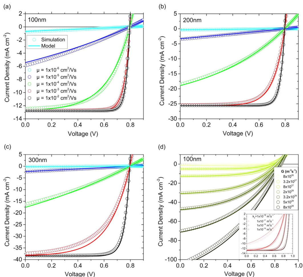
Figure 1. Comparison of JV-curves from 1D DD simulations (symbols) and the analytical approximation (lines) according to Eq. 10. Simulations were performed with the parameters listed in Table S1 and the very same parameters were used to calculate the value of \alpha according to Eq. 12. Only balanced mobilities are considered here. In Figure (a–c), the nongeminate recombination parameter k_2 was set to 10^{-11} cm 3 s -1 and the generation rate G was 8 \times 10^{27} m -3 s -1 , independent of free carrier mobility and active layer thickness. (d) displays simulations and calculations with d = 100 nm, \mu_c = \mu_h = 10^{-4} cm 2 V -1 s -1 and k_2 = 10^{-11} cm 3 s -1 , but now with G varied over two orders of magnitude (corresponding to illumination conditions between about 0.1 suns to 10 suns for a ca. 2 eV absorption bandgap absorber). The inset displays corresponding results for constant G but variable k_2 .
