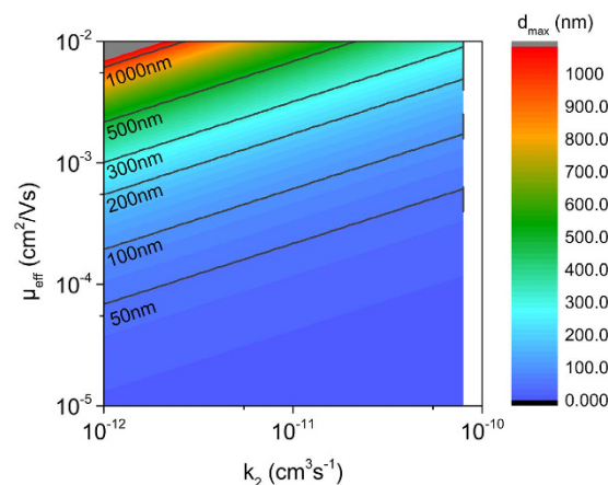
Figure 3. Maximum active layer thickness to avoid transport limitations. Shown is the maximum active layer thickness d_{max} calculated with Eq. 24 in dependence of the effective charge carrier mobility \mu_{eff} = \sqrt{\mu_n \mu_p} and the nongeminate recombination coefficient k_2 for a short circuit current of 15 mA/cm 2 . Above d_{max} , photocurrents become severely transport-limited.
