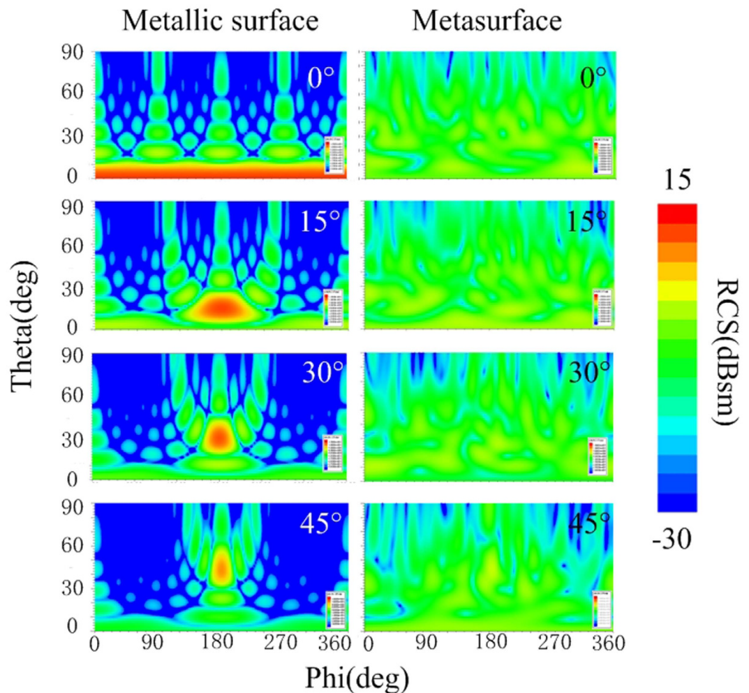
Figure 8. Scattering spectra in the backward space. The spectra are depicted in the same color map scale at 5.86 GHz. The observation area is 0^\circ – 90^\circ in elevation and 0^\circ – 360^\circ in azimuth.
