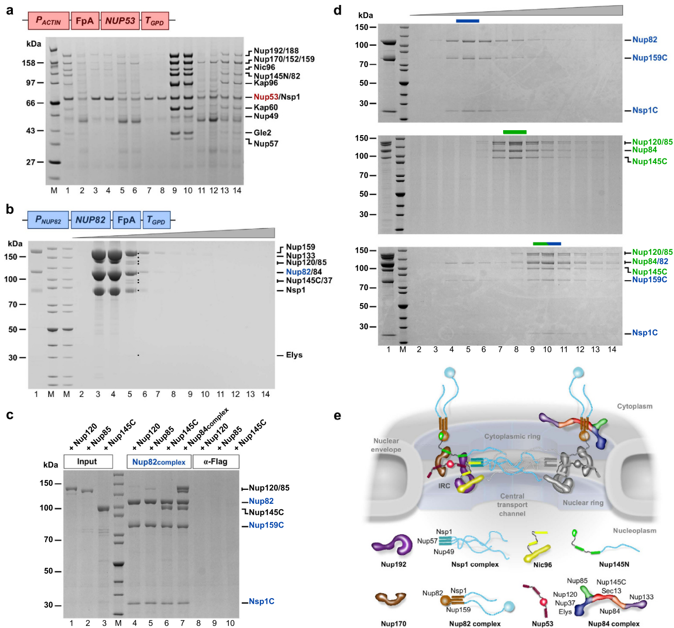
Figure 3. Biochemistry of native C. thermophilum nuclear pore subcomplexes and reconstitution of a Nup82-Nup84 super-complex. (a) Affinity capture of ctNup53 -FpA was performed on cleared lysates under various extraction conditions. Elution of the complexes was followed by SDS-PAGE and Coomassie staining. Proteins identified by mass spectrometric analysis from the complexes isolated in condition #9 are indicated. Extraction conditions (# 1–14) are presented in Supplementary Table 1. A molecular weight marker (M) is indicated on the left. (b) Sucrose gradient centrifugation of the ctNup82 complex upon affinity capture of ctNup82 -FpA. Fractions were collected and analyzed by SDS-PAGE and Coomassie staining. Individual proteins were identified by mass-spectrometric analysis. (c) In vitro binding assay with an immobilized Nup82•Nup159C1•Nsp1C complex ( ctNup82 complex) and full length ctNup120 , ctNup85 and ctNup145C ( ctNup84 complex) (input, lanes 1–3). Samples are eluted via Flag-Peptide and analyzed by SDS-PAGE and Coomassie staining (lanes 5–11). MW: molecular weight, kDa: Kilodalton, \alpha -Flag: Anti-Flag M2 Affinity Gel. (d) Glycerol-gradient centrifugation of in vitro reconstituted complexes. Fractions were collected and analyzed by SDS-PAGE and Coomassie staining. (top) ctNup82 complex, (middle) ctNup84 complex including ctNup84 , (bottom) ctNup82 - ctNup84 complex including ctNup84 . (e) Schematic model for the connection of the Nup53-containing inner pore ring complex (IRC) with the Nup82 outer ring and the Nsp1 channel complex (left) and how the Nup82 complex might be linked to the Y-shaped octameric Nup84 complex within the NPC protomer.
