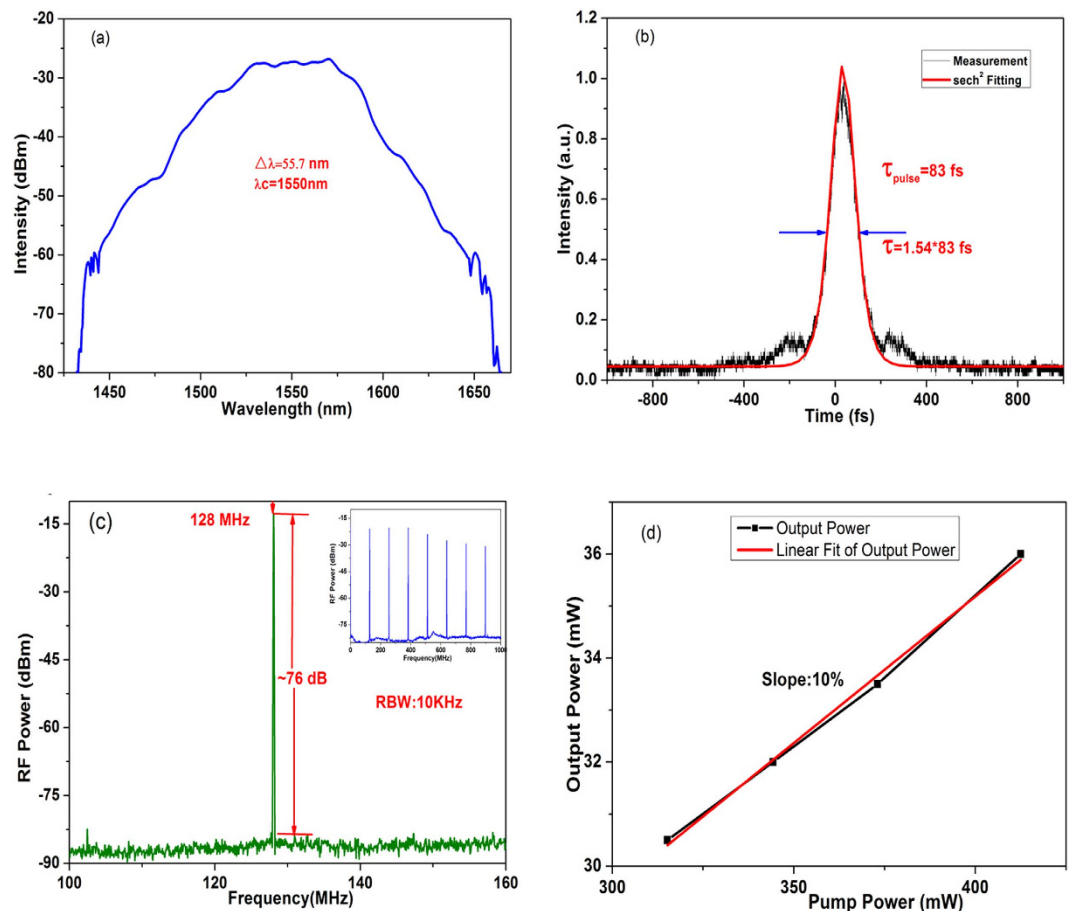
Figure 6. Experimental results of the mode-locked EDF laser without the fiber-taper TI: Sb 2 Te 3 SA. (a) Optical spectrum of the generated pulses, (b) Intensity autocorrelation trace, (c) Radio frequency (RF) spectrum of the mode-locked laser, (d) Laser output power as a function of the pump power.
