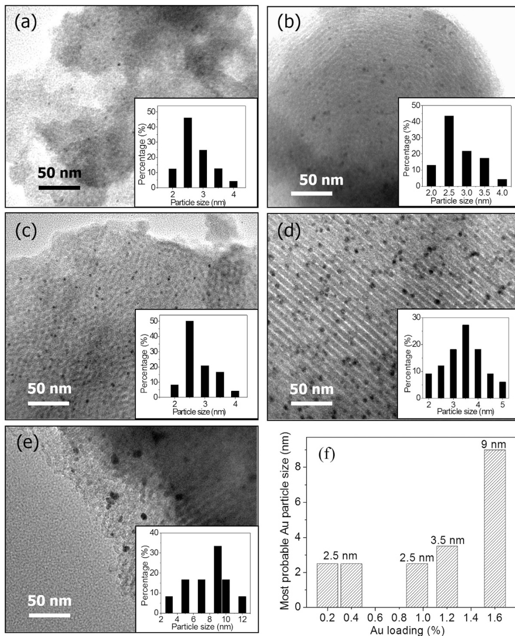
Figure 2. TEM images of catalysts (a) 0.2 wt.%Au/MPTMS-SiO 2 -cal, (b) 0.4 wt.%Au/MPTMS-SiO 2 -cal, (c) 0.95 wt.%Au/MPTMS-SiO 2 -cal and (d) 1.2 wt.%Au/MPTMS-SiO 2 -cal and (e) 1.6 wt.% Au/MPTMS-SiO 2 -cal, (f) the most probable distribution of Au particle size on different Au loading catalysts.
