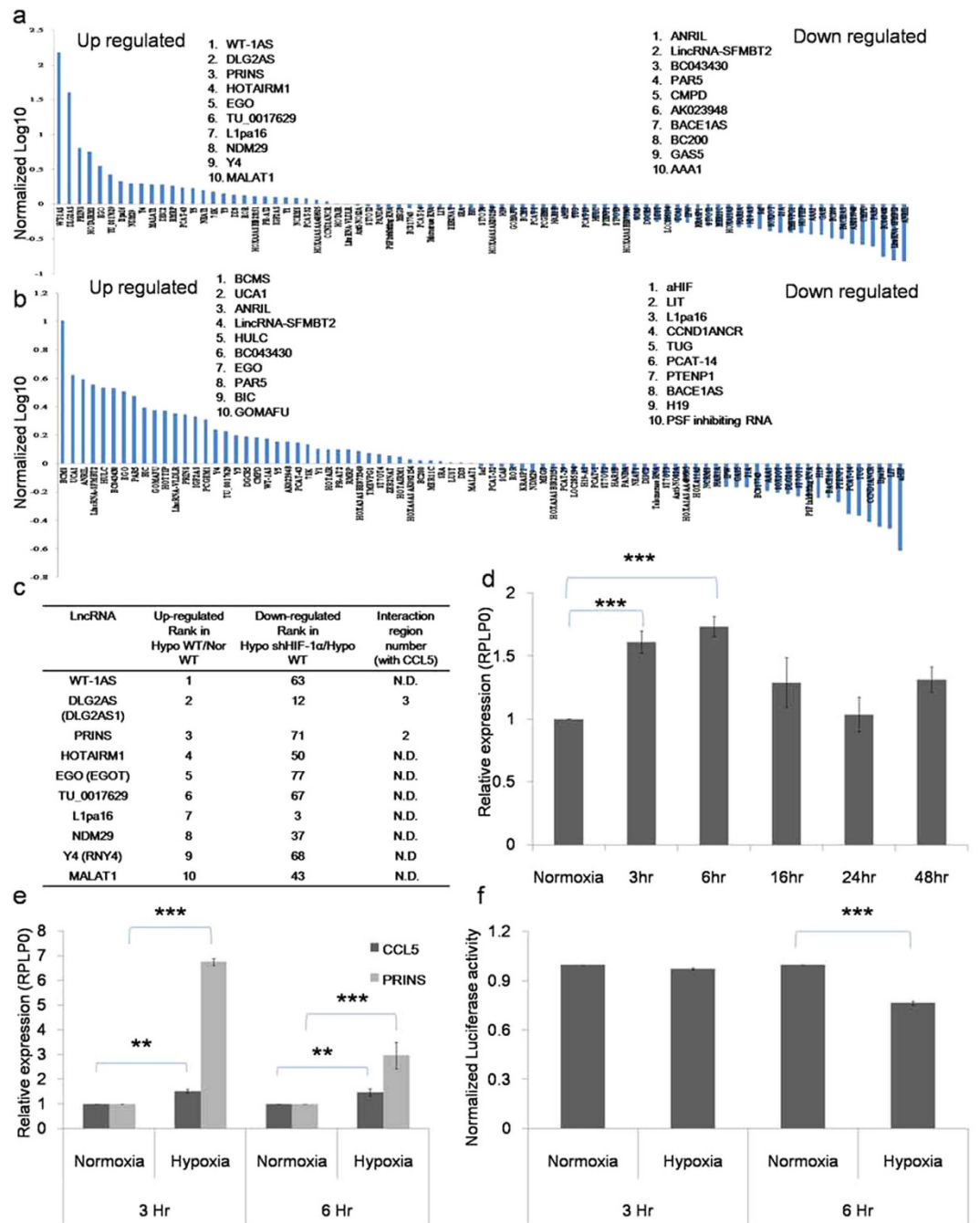
Figure 7. LncRNA-PRINS and RANTES interacts under hypoxia. (a) Deregulated LncRNA in hypoxia/normoxia condition for 24 hours. (b) Deregulated LncRNA in HK-2 sh HIF-1 \alpha and HK-2 cells under hypoxia 24 hours. Briefly, cells were exposed to normoxia/hypoxia for 24 hours, after treatment RNA was isolated and Disease Related LncRNA array was performed. Each bar represents expression of Lnc-RNA relative to internal control. The results show 3 independent experiments performed in triplicates (c) Differentially expressed LncRNA in HIF-1 \alpha dependent manner. (d) Time course study on RANTES mRNA expression by Q-PCR. (e) Q-PCR analysis of RANTES and LncRNA-PRINS under normoxia and hypoxia 3 and 6 hour. Data are expressed as relative levels to RPLP0. The data are shown as the mean \pm SD of three independent experiments performed in triplicates. (f) Luciferase reporter assay: The LncRNA-PRINS luciferase construct vector was transfected into WT-HK-2 cells for 24 hour and incubated under hypoxia and normoxia conditions for 3 and 6 hour respectively. Results were expressed in luciferase activity normalized to Renilla. The data are shown as the mean \pm SD of three independent experiments performed in triplicates.
