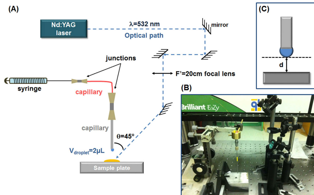
Figure 9. (A) Schematic representation and (B) photograph of the LADC experimental setup. The measurement of the height between the droplet and the sample is schematized in (C).
