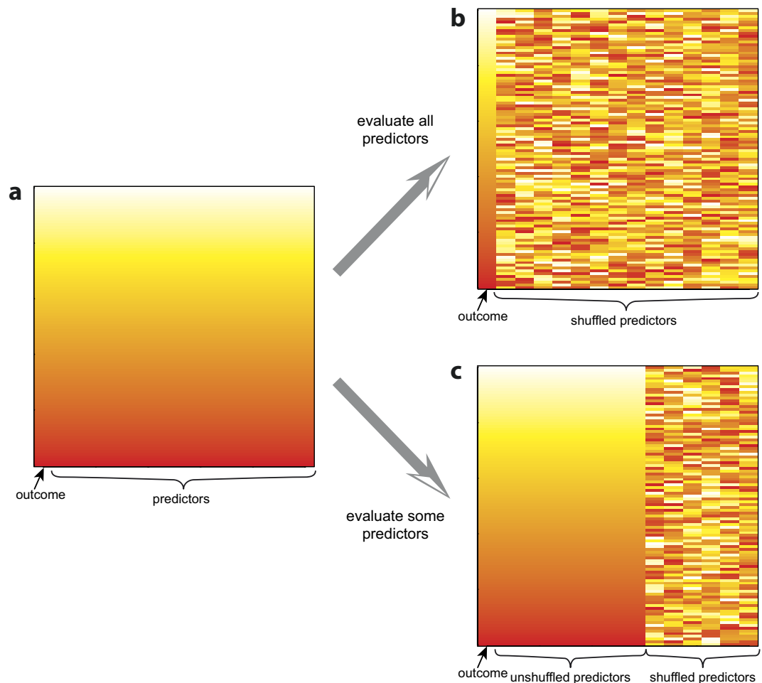
Figure 2. Shuffling methodology for novel Monte Carlo analysis. (a) Graphical representation of a dataset with patient outcome in the leftmost column and the remainder of the columns representing predictor variables; each row is coloured uniquely in a gradient to represent data from an individual patient for illustrative purposes. (b) For the Monte Carlo analysis, the values of each variable are shuffled, randomising that single variable with respect to patient outcome; this is carried out independently for each variable such that correspondence both between a variable and outcome, and among variables, is broken. Note this differs from standard Monte Carlo analyses, which would shuffle only patient outcome with respect to predictors, thus maintaining correspondence among variables. (c) The shuffling procedure can also be performed on a subset of variables, to evaluate only the added value of these variables.
