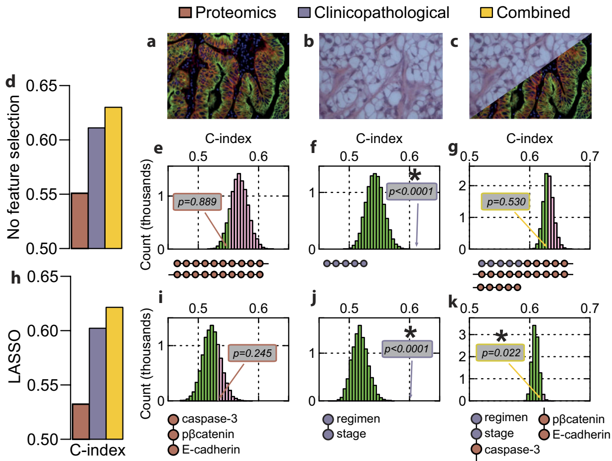
Figure 1. Added value of proteomics for predicting progression-free survival. (a–c) Example images representing proteomics, a fluorescence AQUA image (a) clinicopathology, a histological slice (b) and the combination (c). (d) C-index of Cox proportional hazards regression models for proteomics data only, clinicopathological data only, and combined proteomics and clinicopathological data. (e–g) Corresponding Monte Carlo (MC) analyses showing histograms of c-index from 10,000 randomised datasets; value of the actual analysis is highlighted and its p-value indicated (*-significant); histogram bars are coloured green below the actual value and pink above. (h–k) As for (d–g) after LASSO feature selection; selected features shown below MC histograms in order of decreasing hazard ratio. Note only proteomics data was randomised in (g) and (k).
