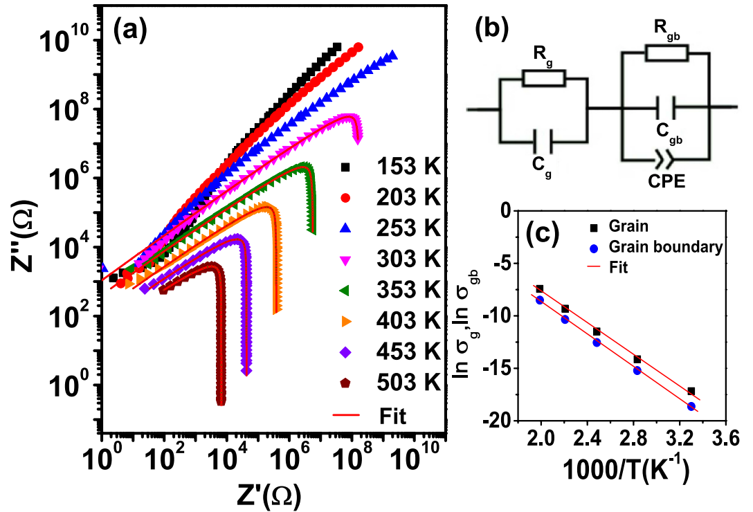
Figure 7. (a) Log-log plots of complex impedance ( Z' vs Z'' ) at different temperatures, (b) equivalent circuit based on the brick-layer model for the impedance spectra, (c) Arrhenius plots of the dc conductivities for grain and grain boundary obtained from the fitting results of equivalent circuit above 303 K.
