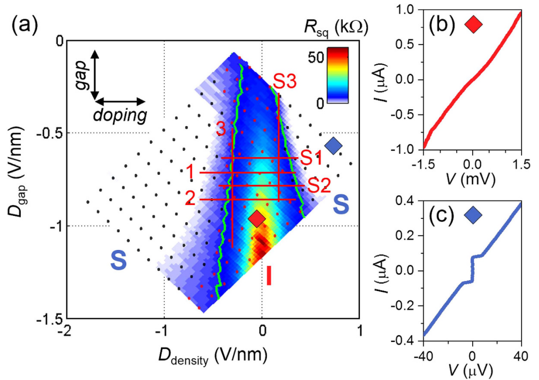
Figure 2. Insulating and superconducting states in an electron-hole puddle system. (a) Color-coded square resistance map of the junction as a function of D_{density} and D_{gap} measured at 50 mK. The diamond symbols indicate representative insulating (red) or superconducting (blue) points of D_{density} and D_{gap} . The green contours correspond to the quantum resistance of Cooper pairs, R_Q = h/4e^2 , and separate insulating regions from the superconducting regions. The red curves indicate gate sweep traces 1–3 and S1–S3. Current–voltage characteristics taken at the corresponding points denoted in (a) exhibit (b) a nonlinear insulating behavior (the red curve) and (c) zero-resistance superconducting behavior (the blue curve).
