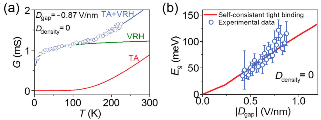
Figure 6. Thermal activation and variable range hopping conduction at the charge neutrality point.
