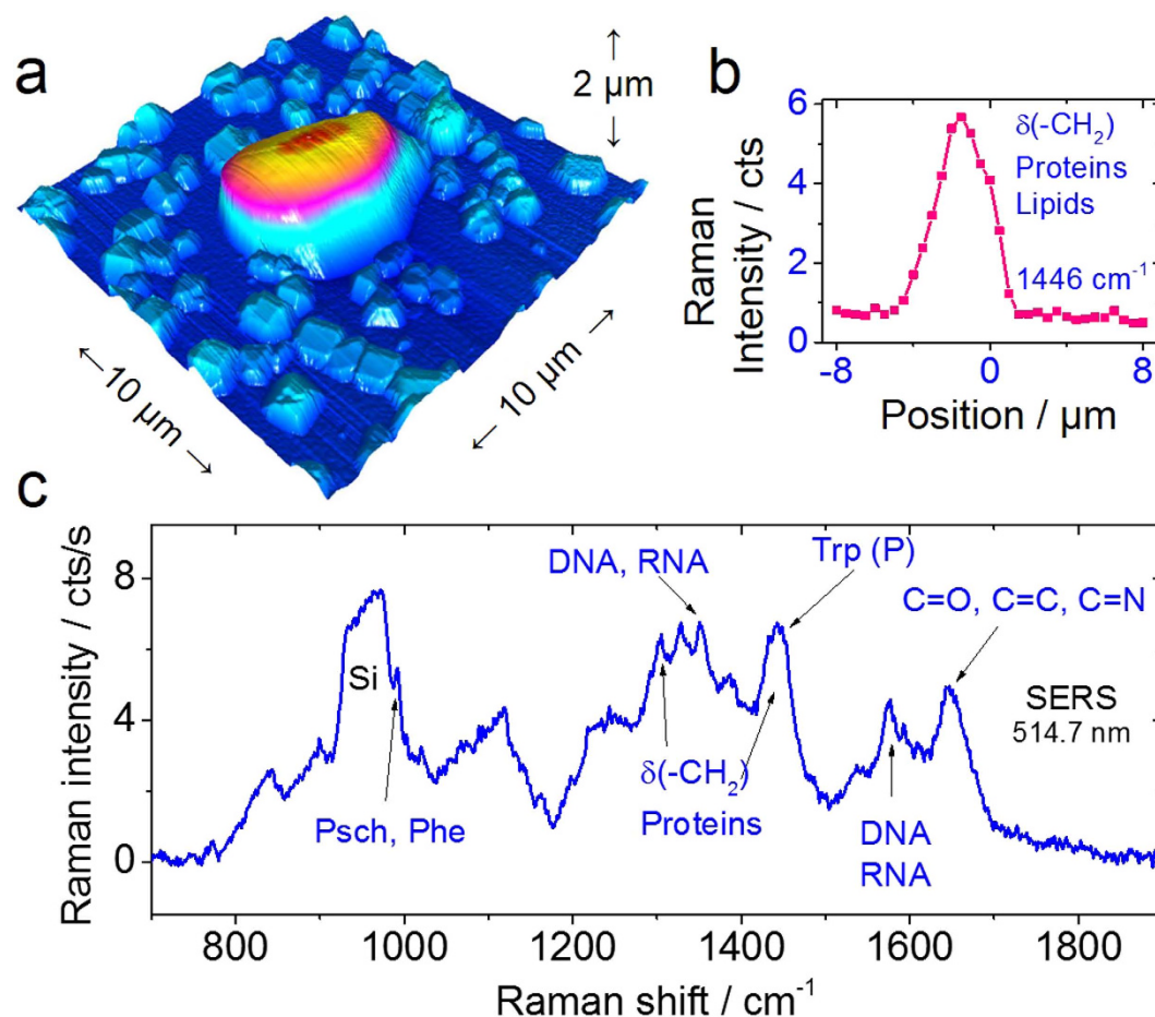
Figure 5. (a) Atomic force microscopy image of a single cell on the silver nanoparticle substrate. (b) Raman line scan showing the spatial distribution of the \text{CH}_2 vibration at 1446\text{ cm}^{-1} related to proteins and lipids. (c) Raman spectrum of a single cell using SERS, the high enhancement even makes the bands visible at the same level as the silicon substrate allowing the observation of the phenyl band that was previously masked. No substrate background subtraction was performed in this case.
