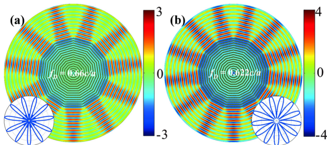
Figure 6. Large-beam Dirac directional emission in photonic crystals. (a) Eleven-beam directional emitter in photonic crystal with 32.7^\circ rhombic lattice. The parameters are r = 0.186a and \varepsilon = 12.5 . (b) Thirteen-beam directional emitter in photonic crystal with 26.7^\circ rhombic lattice, and the parameters are r = 0.156a and \varepsilon = 20 . Blue curves in the insets are the corresponding far-field profiles in linear scale bar.
