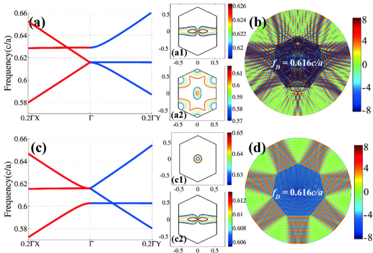
Figure 5. Seven-beam Dirac directional emission in photonic crystals with 51.4^\circ rhombic lattice.
