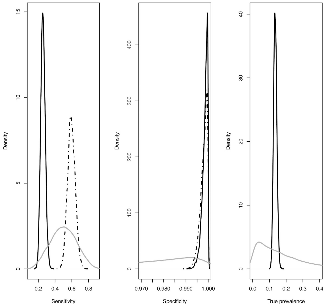
Figure 1. Estimated posterior distributions of parameters from the conditional independence model with outbreak specific diagnostic sensitivities from the Northern Ireland bovine tuberculosis surveillance data. The plots depict the posterior distributions of diagnostic sensitivity and specificity of the single intradermal comparative tuberculin test (broken black line) and abattoir inspection (black line), and average true prevalence from the three Markov chain Monte Carlo chains run. The grey lines represent the prior distributions used to inform the estimates. The x-axis provides the parameter estimates and the y-axis the relative probability of taking a given value.
