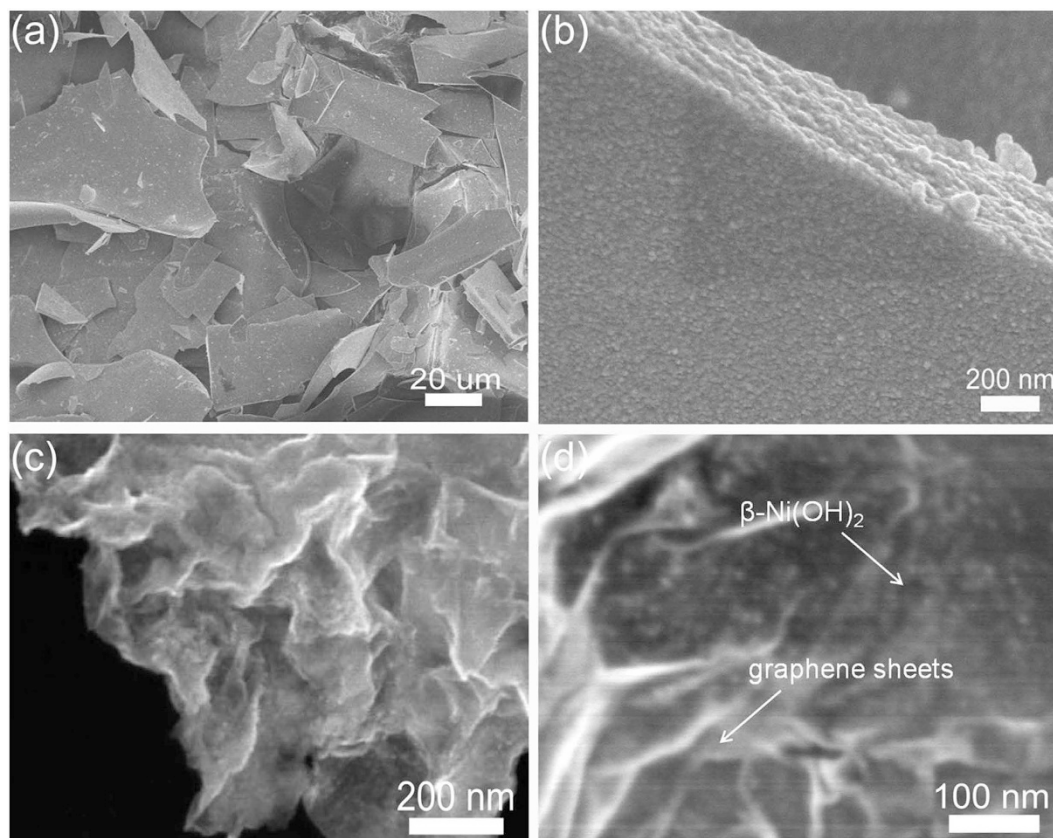
Figure 4. SEM images of the pure \text{Ni(OH)}_2 and RGO- \text{Ni(OH)}_2 composite: (a and b) low and high magnification SEM images of \text{Ni(OH)}_2 sheets, and (c and d) low and high magnification SEM images of RGO- \text{Ni(OH)}_2 composite.
