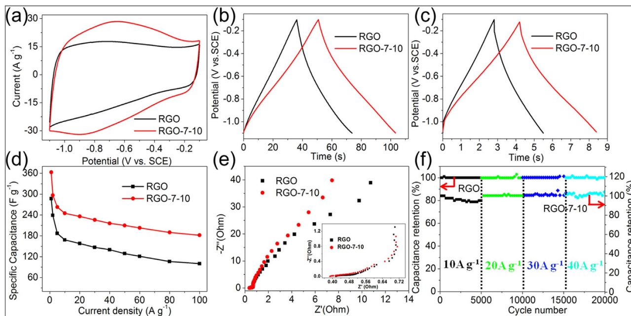
Figure 7. (a) CV curves of RGO and RGO-7-10 at a scan rate of 100 mV s -1 . (b and c) GCD curves of RGO and RGO-7-10 at current densities of 5 and 50 A g -1 , respectively. (d) The specific capacitance as a function of current density for RGO and RGO-7-10. (e) Nyquist plots of RGO and RGO-7-10. Inset shows the close-up view of the high-frequency regime. (f) Cycling stability of RGO and RGO-7-10 at different current densities of 10 A g -1 , 20 A g -1 , 30 A g -1 and 40 A g -1 , respectively. The running cycle at each current density is the same as 5 000 cycles.
