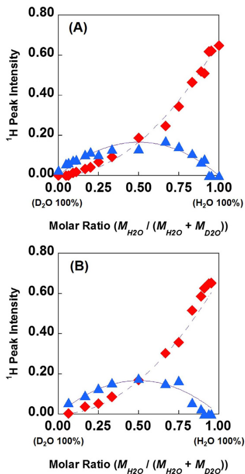
Figure 4. Peak intensity changes of the water peaks in the ^1\text{H} NMR spectrum of (A) [DEME][BF 4 ] and (B) [BMIM][BF 4 ]/50 mol% water mixtures as the \text{H}_2\text{O} : \text{D}_2\text{O} molar ratio is varied in a 50 mol% water mixture. Legends: \blacklozenge = de-shielded water peak intensity, \blacktriangle = shielded water peak intensity, dashed line = theoretical value of total \text{H}_2\text{O} peak intensity, solid line = theoretical value of total HOD peak intensity. Note that H/D exchange reaction between the exchangeable proton and water does not occur in this condition (pH4.88–5.73).
