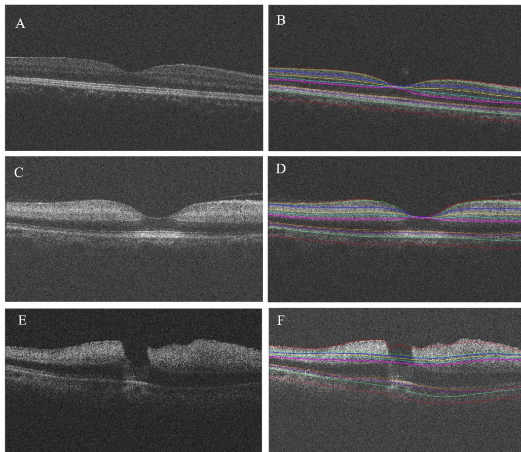
Figure 1 | Segmented surfaces and regions on macular spectral domain optical coherence tomography. (A,B.): control subjects; (C,D.): central retinal artery occlusion patients with correctly segmented retinal layers; (E,F.): central retinal artery occlusion patients with substantially increased brightness of the inner retina and related insufficient separation of inner retinal layers on OCT, causing layer segmentation errors – an example is shown. (A,C,E): original OCT images; (B,D,F): segmentation results.
