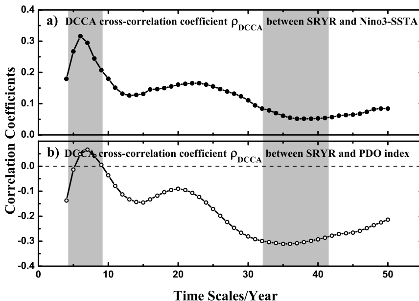
Figure 2 | DCCA cross-correlation coefficient \rho_{DCCA} between SRYR and Nino3-SSTA (a), as well as SRYR and PDO index (b). The grey region covers the time scale of 5 ~ 8 years (El Niño typical scale) and the time scale of 33 ~ 42 years (PDO typical scale). The two curves have similar pattern.
