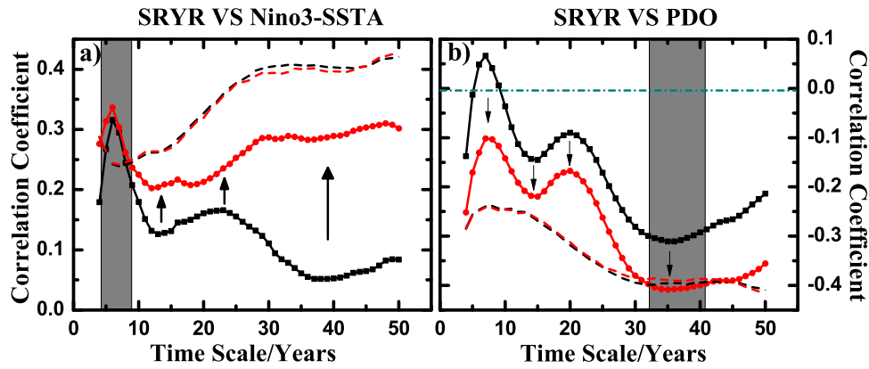
Figure 5 | Application of DPCCA to the climatic example. DCCA (black) and DPCCA (red) outputs between (a) SRYR and Nino3-SSTA, (b) SRYR and PDO. The black dashed line represents the 95% significance criterions of \rho_{DCCA} on different time scales, while the red dashed line represents the criterions of \rho_{DPCCA} . They are both obtained from Monte-Carlo Simulations according to 45 . We shuffled the considered time series and repeated the DCCA/DPCCA calculations for 10,000 times. The top 2.5% largest values (on different time scales) give the dashed lines in (a), while the top 2.5% smallest values give the dashed lines in (b). The grey area covers the typical time scales where (a) the Nino3-SSTA has significant positive correlation with SRYR on time scales of 5 ~ 8 years, and (b) the PDO has significant negative correlation with SRYR on time scales of about 35 years.
