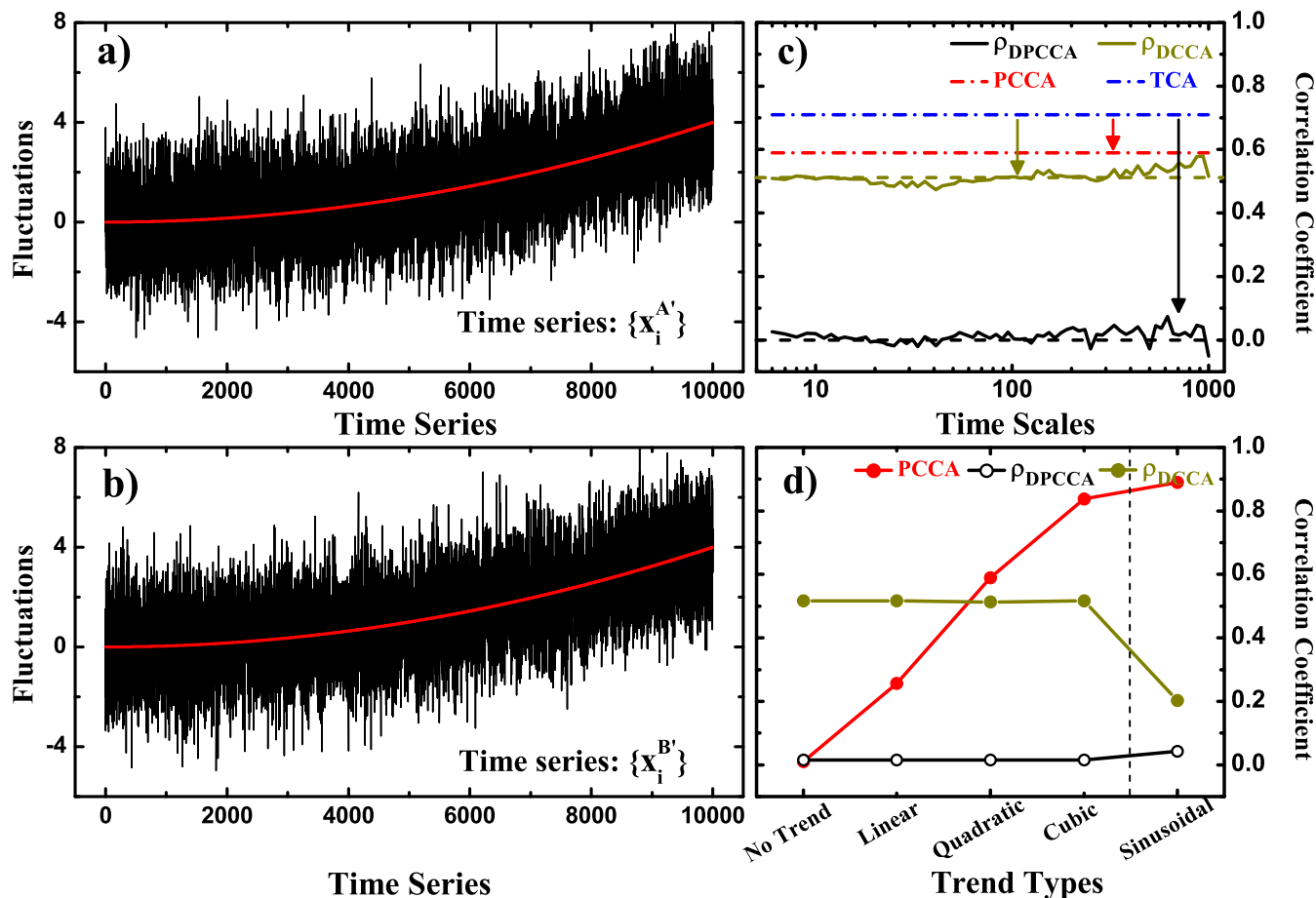
Figure 3 | Time series and related results in Test I. (a, b) show the two time series \{x_i^{A'}\} and \{x_i^{B'}\} in test I, but with quadratic trends. The results of traditional cross-correlation analysis (TCA, blue), partial cross-correlation analysis (PCCA, red), detrended cross-correlation analysis (DCCA cross-correlation coefficient \rho_{DCCA} , yellow), as well as the detrended partial-cross-correlation analysis (DPCCA, black) are shown in (c). In (d), more cases with higher-order trends are shown. For each “Trend Type”, the detrend order of DPCCA (DCCA) are different, as DPCCA1 (DCCA1), DPCCA2 (DCCA2), DPCCA3 (DCCA3), DPCCA4 (DCCA4), and DPCCA16 (DCCA16), respectively. The coefficient of each “Trend Type” is actually the mean correlation coefficient averaged over all the time scales in (c).
