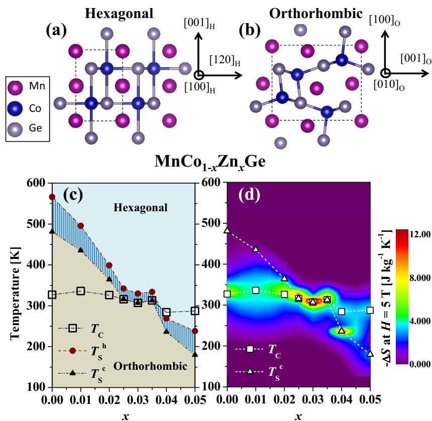
Figure 1 | Magnetic- and structural-phase-diagram. Schematic figure of the (a) hexagonal and (b) orthorhombic structure of \text{MnCoGe} as viewed along the same spatial direction. Dashed lines indicate unit cells for the respective structures. The directions of crystal axes are indicated with conventional hexagonal and orthorhombic settings, respectively. (c) Magnetic and structural phase diagram of \text{MnCo}_{1-x}\text{Zn}_x\text{Ge} . The hatched area indicates the thermal hysteresis related to the structural transition. T_S^h and T_S^c denote structural transition temperatures on heating and cooling, respectively. T_C indicates ferromagnetic transition temperature on cooling. (d) Contour plot of the magnetocaloric effect, or equivalently isothermal entropy change ( -\Delta S ), of \text{MnCo}_{1-x}\text{Zn}_x\text{Ge} for a field change from 0 T to 5 T which was measured in the cooling run.
