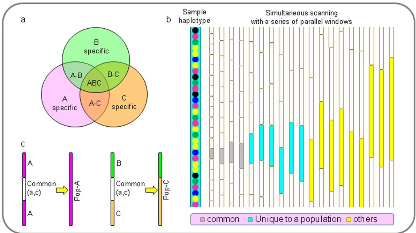
Figure 3 | The aMAP algorithm. (a) Reference analysis and pretreatment prior to use. (b) Parallel window scan using a set of parallel sliding windows and horizontal data integration. (c) Vertical data integration that integrates local ancestral calls from adjacent windows. Common calls are indicated by brackets.
