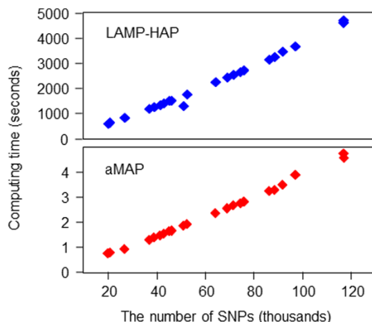
Figure 2 | The computing time of aMAP and LAMP. The whole-genome of 20 HapMap ASW individuals (African-Americans) were analyzed with three references (CEU, YRI, and CHBCHD). The computing speeds of aMAP and LAMP-HAP are compared, and both are linear to the total number of SNPs; the speed of aMAP is about 923 times faster than the speed of LAMP-HAP.
