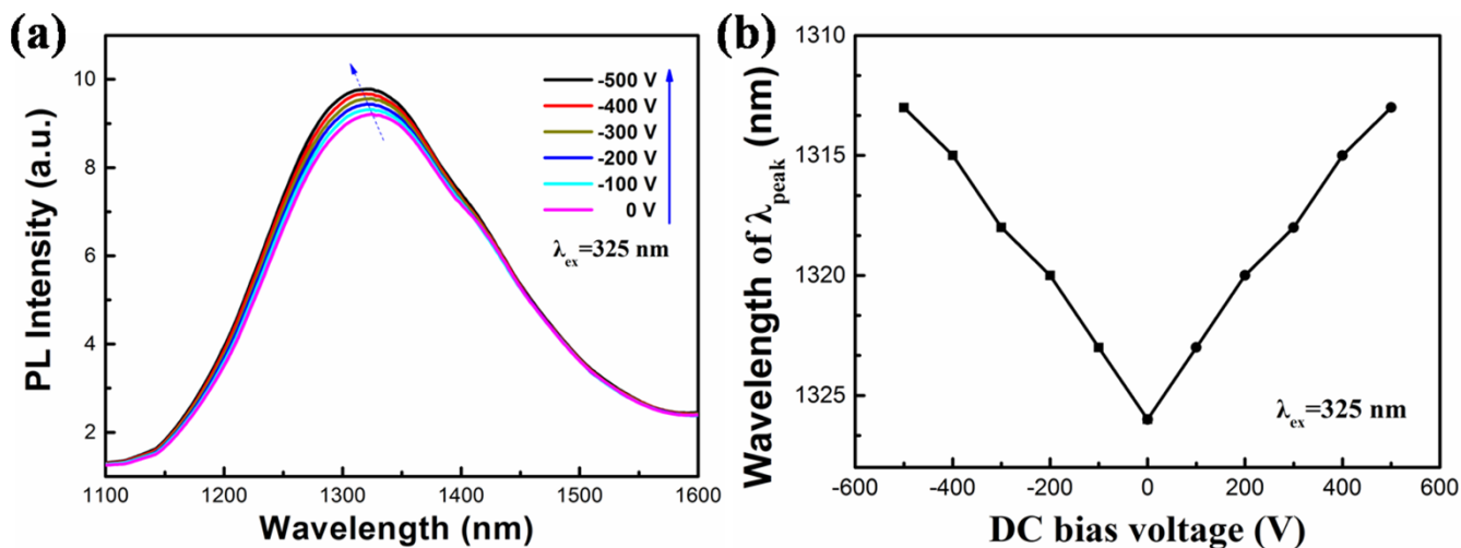
Figure 6 | (a) The PL spectra of STO:Ni (600 nm)/PMN-PT with 325 nm excitation, under DC bias voltage changed from 0 to -500 V. (b) The PL emission peak position of STO:Ni (600 nm)/PMN-PT as a function of the applied voltage from -500 V to 500 V.
