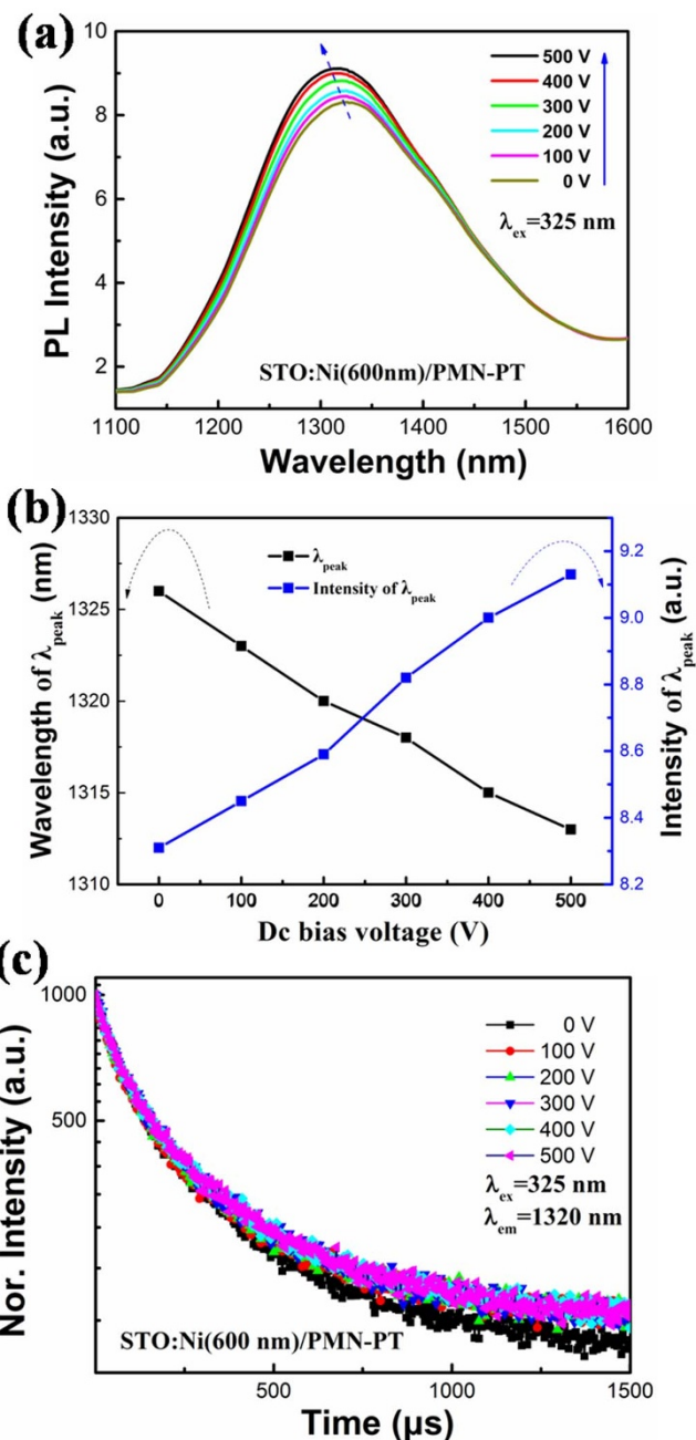
Figure 4 | The PL results of STO:Ni (600 nm)/PMN-PT under 325 nm excitation, when DC bias voltage is applied from 0 to 500 V. (a) The PL spectra of STO:Ni (600 nm)/PMN-PT. (b) The summarized PL results of STO:Ni (600 nm)/PMN-PT. (c) The NIR PL decay curves of STO:Ni (600 nm)/PMN-PT.
