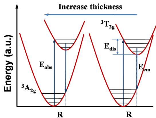
Figure 3 | Configurational coordinate diagrams for STO:Ni samples. The lowest electronic states {}^3A_{2g} are shown; Horizontal lines represent vibrational energy levels. The upward and downward arrows indicate absorption and emission transitions, respectively. R is the distance between Ni^{2+} ions and ligands. E_{dis} represents the difference between the excited state vibrational level reached in the absorption transition and the minimum level of the same state.
