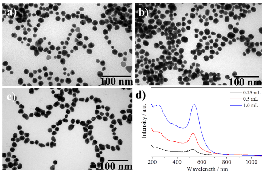
Figure 2 | TEM images of the Au NPs prepared by the reaction of 0.25-mL a), 0.5-mL b), and 1-mL c) \text{HAuCl}_4 (5 mM) with 10 mL of PSMA polymer (0.78 mg/mL) at 200^\circ\text{C} for 1 h. d) UV-visible spectra for these corresponding Au NPs.
