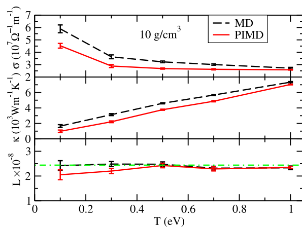
Figure 5 | Electrical conductivity, thermal conductivity and Lorenz number of dense hydrogen as a function of temperature at 10 g/cm 3 . For Lorenz number, the dot-dashed line denotes the value of the degenerate limit 2.44 \times 10^{-8} \Omega \text{WK}^{-2} .
