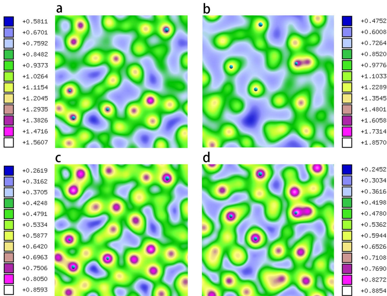
Figure 4 | The cut-plane of 3D distribution of charge density (a, b) and electron localization function (c, d) of randomly selected configurations from MD (a, c) and PIMD (b, d) simulations at 10 g/cm 3 and 0.3 eV. In PIMD calculations, the configuration is randomly selected from imaginary-time slices in PIMD time steps. Note that with the inclusion of NQEs, the charge density and electron localization function have the larger maxima and smaller minima compared to the classical simulations. It indicates that electrons surrounding ions distribute more localized with quantum nuclei than classical particle treatment. All the other randomly selected configurations exhibit the same behavior as the example presented here.
