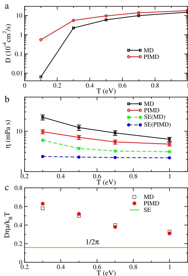
Figure 1 | Temperature dependence of the self-diffusion coefficient (a) and shear viscosity (b) at 10 g/cm 3 obtained from centroid PIMD and MD simulations. The viscosities obtained from the Stokes-Einstein (SE) relation are also presented. (c) Examination of SE relation with respect to temperature. The effective atomic diameter in SE relation is defined by the position of the first peak of radial distribution function.
