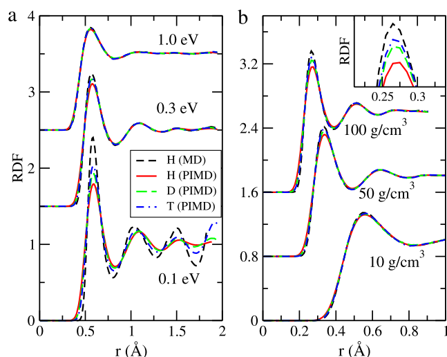
Figure 2 | Radial distribution functions of hydrogen nuclei from PIMD (solid lines) and MD (dashed lines) simulations with different temperatures at 10 g/cm 3 (a), and with different densities at 1 eV (b). The isotopes effects of deuterium (D) (long-dashed lines) and tritium (T) (dot-dashed lines) are also presented. The inset is the first peak of radial distribution functions at 100 g/cm 3 and 1 eV.
