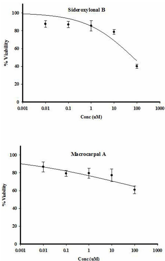
Figure 3 | Dose response curve of Sideroxylylonal B (A) and Macrocarpal A (B) against MCF-7 cell line fitted to E_{max} model.
