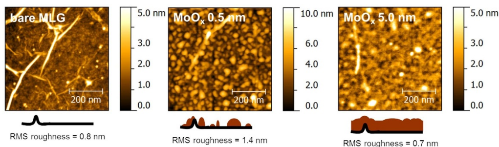
Figure 4 | AFM images measured in non-contact mode of (a) as transferred monolayer graphene, (b) + 0.5 nm MoO 3 and (c) + 5 nm MoO 3 . Schematic sketches are not to scale.
