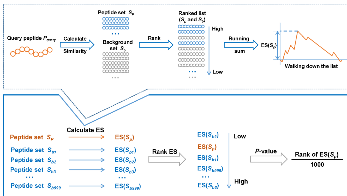
Figure 6 | Detailed processes of the PSEA method.
