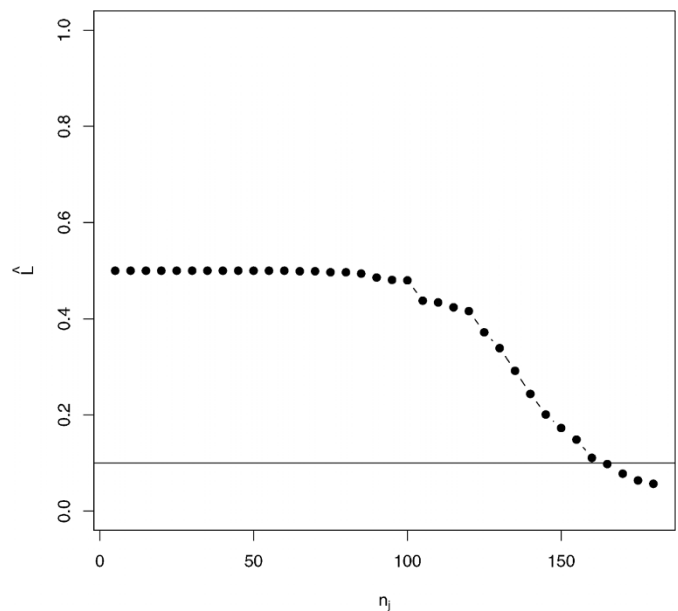
Figure 1 | C. elegans graph classification simulation results. The estimated hold-out misclassification rate \hat{L}_F^n(g_n) (with n' = 1000 testing samples) is plotted as a function of class-conditional training sample size n_j = n/2 , suggesting that for \varepsilon = 0.1 we can determine that \mathcal{M}^{\varepsilon}_F \mathcal{B} holds with 99% confidence with just a few hundred training samples generated from F_{MB} . Each dot depicts \hat{L}_F^n(g_n) for some n ; standard errors are (\hat{L}_F^n(g_n)(1 - \hat{L}_F^n(g_n))/n')^{1/2} . For example, at n_j = 180 we have k_n = \lfloor \sqrt{8n} \rfloor = 53 (where \lfloor \cdot \rfloor indicates the floor operator), \hat{L}_F^n(g_n) = 0.057 , and standard error less than 0.01. We reject H_0^{0.1} : L^* \geq 0.1 at \alpha = 0.01 . Note that L^* \approx 0 for this simulation.
