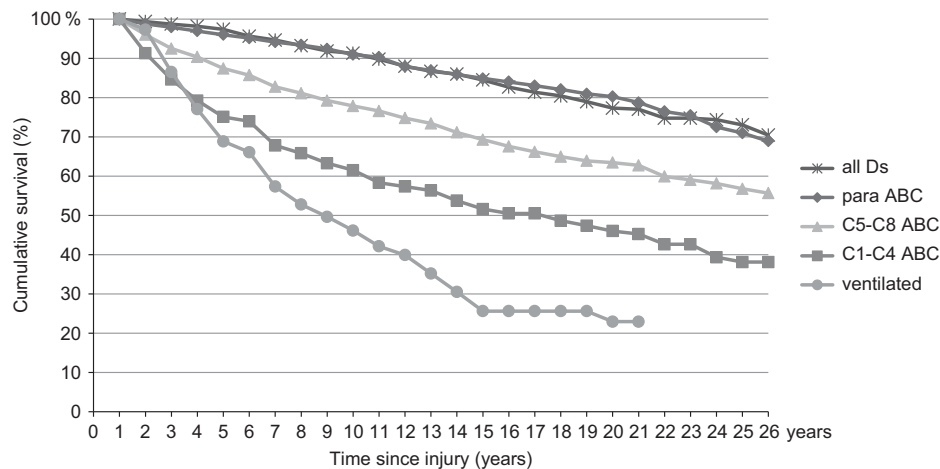
Figure 1 Cumulative 25 year survival curve versus time since injury for 1980–2014 study period by five neurological groups. A full color version of this figure is available at the Spinal Cord journal online.
