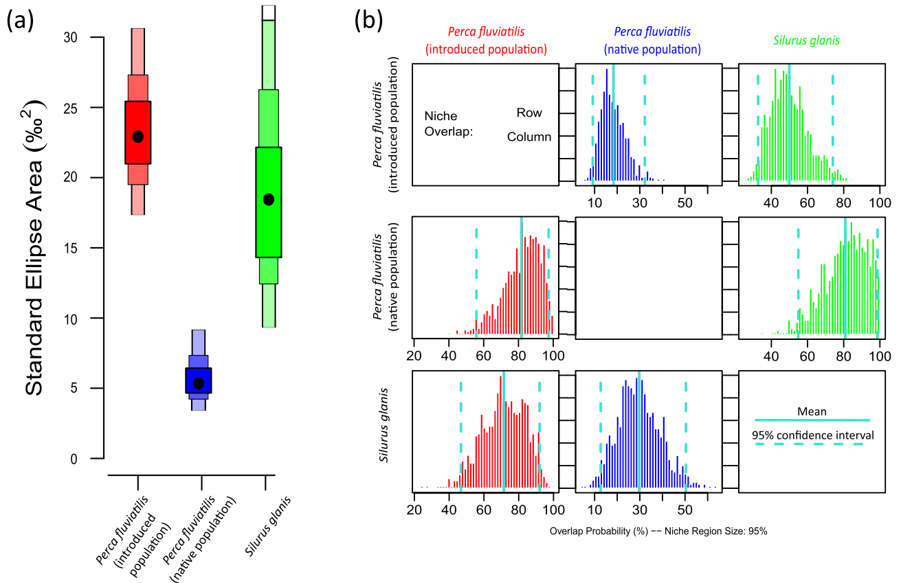
Figure 3. A posteriori distributions for the Bayesian standard ellipse areas (SEAb) (a) and the niche overlap based on the 95% confidence interval (SEAb) (b) for native Perca fluviatilis from lakes, introduced P. fluviatilis from reservoirs, and Silurus glanis native to İznik Lake.
