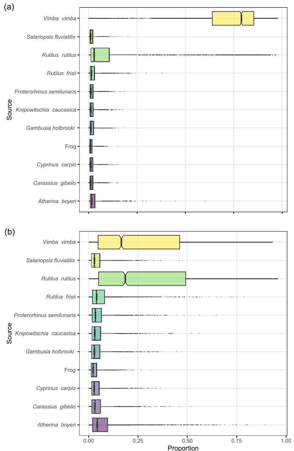
Figure 2. Mixing models results for (a) introduced perch vs (b) native perch.
