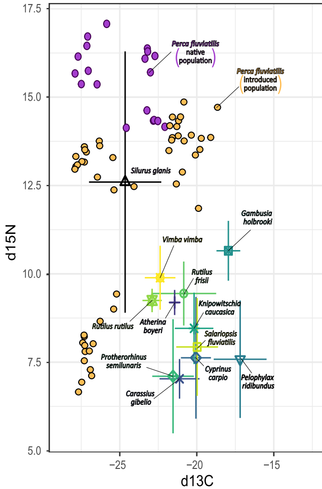
Figure 1. Carbon ( \delta^{13}\text{C} ) and nitrogen ( \delta^{15}\text{N} ) stable isotopes biplot of the İznik Lake fish community, with potential prey species for native and possibly introduced Perca fluviatilis .
