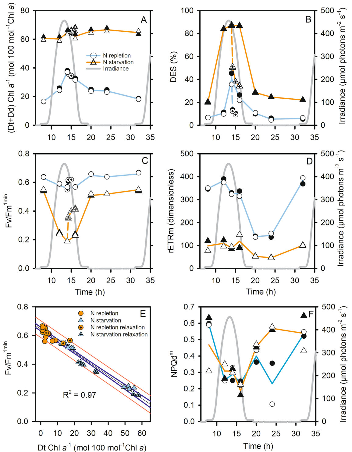
Figure 3. Time dependent change in (\text{Dd} + \text{Dt})/\text{Chl } a (A), de-exposition ratio ( \text{DES} = \text{Dt}/(\text{Dd} + \text{Dt}) \times 100 ) (B), \text{Fv}/\text{Fm}^{1\text{min}} (C), rETRm (D) and \text{NPQ}_d^m (F) during a diel cycle and relationship between \text{Fv}/\text{Fm}^{1\text{min}} and \text{Dt}/\text{Chl } a (E) in N-sufficient (circles) and N-starved growth (triangles). In A, B, C, and E, crossed symbols represent the two replicates of the relaxation experiments (incubation in darkness, see the “Methods” and “Results” section). In A, B, C, D and F, a line passes through the mean of the two replicates. The grey line represents growth irradiance.
