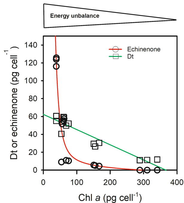
Figure 6. Relationship between Chl a/cell and Dt/cell (squares) and echinenone/cell (circles) in T. lutea . As energy unbalance increase (illustrated in the scale above the graph), Chl a per cell decreases and both diatoxanthin and echinenone increase.
