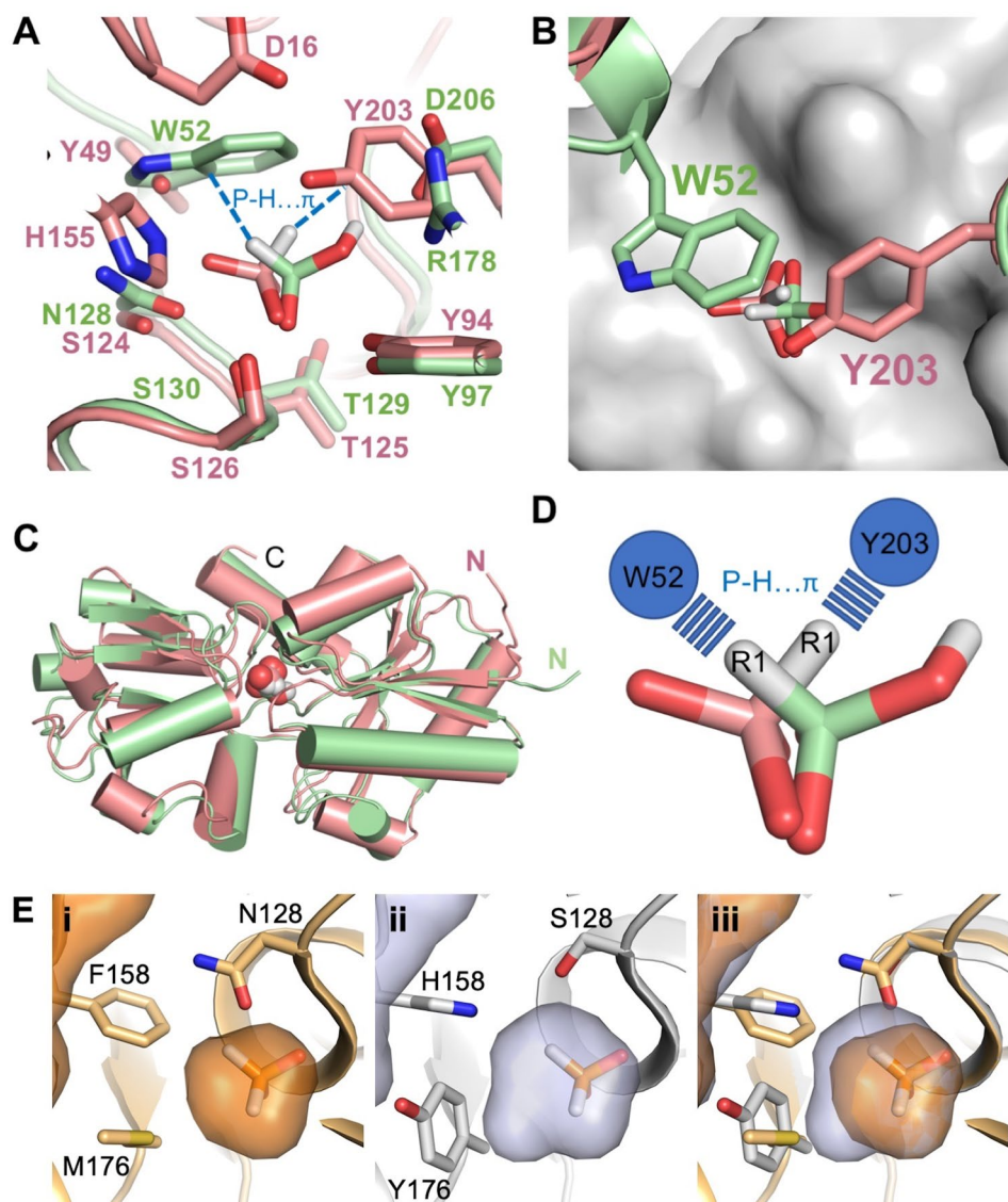
Figure 7. Sequence differences in the binding pocket of related phosphite and hypophosphite PBPs change the shape and orientation of the ligand binding site. (A) Sequence conservation in the binding pocket and mode of binding of phosphite in HtxB (green) and PtxB (pink). The protein is drawn as a cartoon, with the ligands and side chains drawn as sticks. The P-H... \pi interaction is drawn as a blue dashed line. (B) A view of the relative orientation of the \pi system that provides ligand specificity. The view is rotated 90° relative to (A) , with the positions of W52 and Y203 shown as sticks above the phosphite. The molecular surface of the binding pocket is shown in grey. (C) The fold and conformation of the two proteins is largely conserved. The protein backbones are represented as a cartoon and the ligands as spheres. (D) The mode of binding of phosphite in HtxB and PtxB are mirror-images of each other. The phosphite molecules are shown as sticks and the relative position and interactions with W52 and Y203 are indicated schematically with circles and dashed lines, respectively. (E) The volume of the binding pocket (shown as an enclosed surface) in (i) HtxB (orange), (ii) modelled HtxB-hybrid (grey) and (iii) an overlay of the two volumes. Sequence differences around the binding pocket generate more space in the hybrid. The position of hypophosphite in the HtxB structure is shown for reference.
