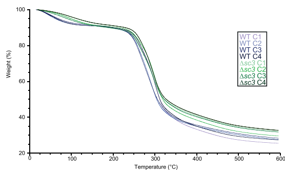
Figure 5. Thermogravimetric analysis of mycelia of S. commune wild type and \Delta sc3 grown in the dark at low (C1) and high (C2) \text{CO}_2 and in the light at low (C3) and high (C4) \text{CO}_2 . Experiments were performed in duplicate.
