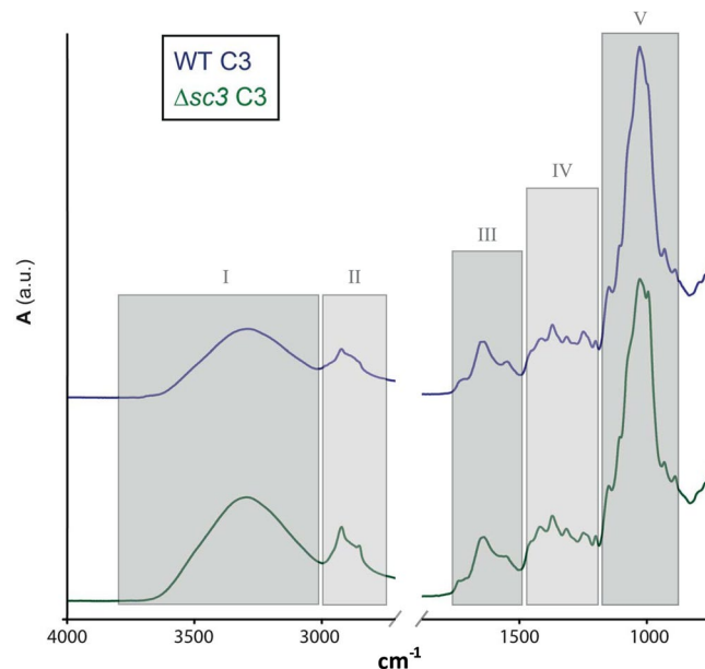
Figure 4. ATR-FTIR spectra of liquid static cultures of S. commune wild type and \Delta sc3 grown in light and low \text{CO}_2 . Similar absorption peaks were observed between strains, indicating that the mycelia had a similar chemical composition. Definition of wavenumber regions I-V can be found in Table 2. Spectra were obtained in quadruple.
