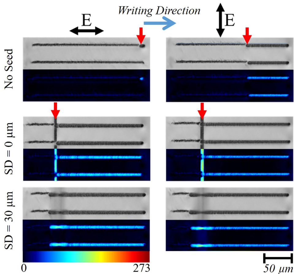
Figure 3. Instigating the damage-like modification to self-assembled nanograting transition with seed lines at different seed depths (SD). 200 \mu\text{m} length lines written at 1 mm/s with 3.5 \mu\text{J} pulses. Regardless of the SD, the transition (red arrows) occurs when the laser line hits the pre-written seed, instigating the transition earlier than when there is no seed present. As the laser light interacts with the pre-written seed, the light is scattered effectively acting as a drop in pulse energy during laser writing. The drop in pulse energy experienced illustrates how minor fluctuations instigate the process.
