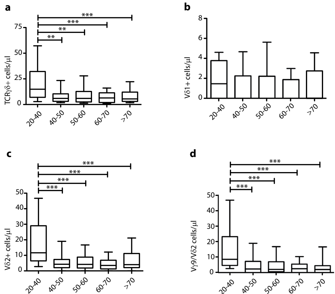
Figure 1. V\gamma/V\delta -gene usage in TCR\gamma\delta+ T-cells in different age groups. (a) Absolute numbers of total TCR\gamma\delta+ T-cells, (b) V\delta1+ , (c) V\delta2+ and (d) V\gamma9/V\delta2 TCR\gamma\delta+ T-cells depicted as 10–90% box-whisker-plots. Significance was tested by a Kruskal-Wallis test, followed by a post-Dunn's test to correct for multiple testing. Significance for the Dunn's test is indicated in the plots: ** p < 0.01 ; *** p < 0.001 .
