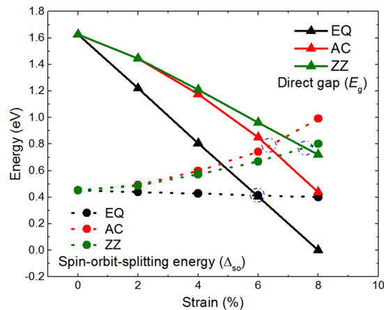
Figure 4. Calculated direct gap ( E_g ) and spin-orbit-splitting energy ( \Delta_{so} ) at \Gamma point of stanane as fractions of biaxial strain along EQ direction, uniaxial strain along AC and ZZ directions. The solid and dash lines represent E_g and \Delta_{so} , respectively.
