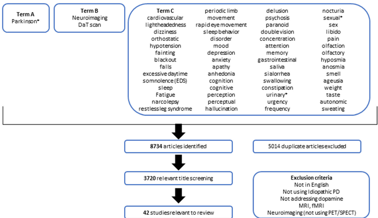
Fig. 2 Methodology used for this review. DaT dopamine transporter, EDS excessive daytime somnolence, MRI magnetic resonance imaging, fMRI functional MRI, PET positron emission tomography, SPECT single positron emission computed tomography, PD Parkinson's disease
