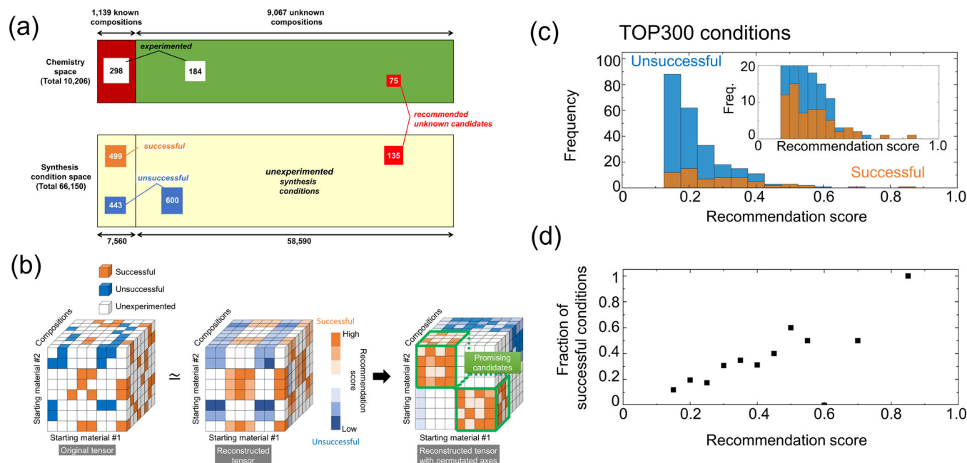
Fig. 7 | A synthesis-condition recommender system. a The chemistry space and the synthesis condition space. b A schematic of the Tucker decomposition of the synthesis condition tensor. c Results of additional synthesis experiments for the top 300 synthesis conditions. The number of successful (orange) and unsuccessful (blue) results were shown as a function of the recommendation score. d The fractions of the successful synthesis conditions, i.e., success rate, for each bin of the recommendation score in c . Adopted from ref. 32 with small modifications.
