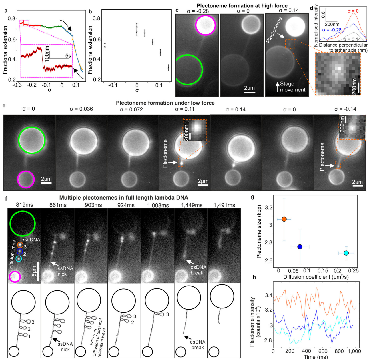
Fig. 5 | Plectoneme dynamics in single molecules. a 1.0 pN continuous asymmetric hat curve, SYBR Gold added (arrows indicate red-green-blue overtwin followed by yellow undertwin, drift-corrected). Inset: Zoom-in (red) plus black running 1500-point median filter. b 0.5 pN discontinuous hat curve showing extension reduction during positive/negative supercoiling (optical resolution error bars \pm 0.03 fractional extension), n=1 . c Fluorescence microscopy of 1 pN pleconeme formation at \sigma = -0.28 (no pleconeme), 0 (no pleconeme) and 0.14 (inset pleconeme), one representative example. d Line profiles for tethers of (c) normalised to \sigma = 0 spanning blur region of \sigma = -0.28 tether using same size region for \sigma = 0 and \sigma = 0.14 tethers but excluding pleconemes, indicating FWHM of 251, 214, 205 nm for \sigma = -0.28, 0, 0.14 respectively (s.d. error 0.2%, “Methods” section). e One representative tether from fluorescence microscopy, low force pleconeme formation, anchor/magnetic bead indicated with green/magenta circles: when DNA overtwisted a pleconeme forms/grows (inset, with altered display settings to match local background). Removing positive supercoiling allows DNA to relax,
