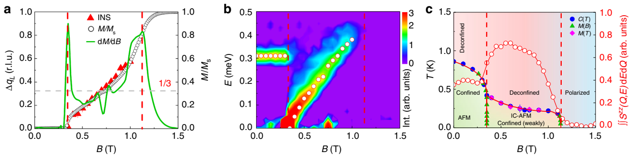
Fig. 6 Field-dependent magnetization and magnetic phase diagram of \text{YbAlO}_3 . a Field-dependent zero energy soft point at wave vector shift \Delta q_L = Q_L - 1 , extracted from the INS. Normalized magnetization M/M_s , measured at 0.05 K, and the corresponding magnetic susceptibility dM/dB are over plotted. M_s is the saturation magnetism for fields along the a -axis, and the horizontal dashed lines indicate the 1/3 magnetization plateau. b Field evolution of the energy-dependent inelastic neutron spectrum, at 0.05 K, integrated over wave vector H = [-0.1, 0.1] r.l.u., K = [-0.6, 0.2] r.l.u., L = [0.9, 1.1] r.l.u.. The empty circles indicate the peak positions. c The field-temperature ( B - T ) magnetic phase diagram. The field-dependent INS spectrum measured at 0.05 K is over plotted, which is integrated over H = [-0.1, 0.1] r.l.u., K = [-0.6, 0.2] r.l.u., L = [0, 2] r.l.u., and E = [0.05, 0.6] meV. The vertical dashed lines indicate the critical field B_c = 0.35 T, and saturation field B_s = 1.13 T, defined through the peak positions of dM/dB
