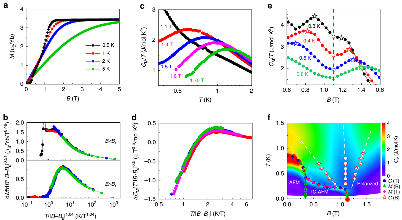
Fig. 7 Quantum critical scaling and universality of \text{YbAlO}_3 . a Field-dependent magnetization M measured at different temperatures. b Critical scaling of the magnetic susceptibility in a , for fields both below and above B_s . c Temperature-dependent magnetic specific heat C_M/T measured at different fields. d Critical scaling of the field-dependent magnetic specific heat \Delta C_M/T shown in c . e Field-dependent magnetic specific heat C_M/T at different temperatures. The red dashed line indicates the saturation field B_s = 1.1 T at the minimum, and crossovers with two broad maximum shoulders are observed. f Contour plot of the magnetic specific heat C_M as a function of temperature and field. Magnetic phase boundaries extracted through different measurements are over-plotted. The red circles indicate the saturation field B_s at different temperatures, and the empty stars indicate the crossover defined through the field-dependent specific heat maxima
