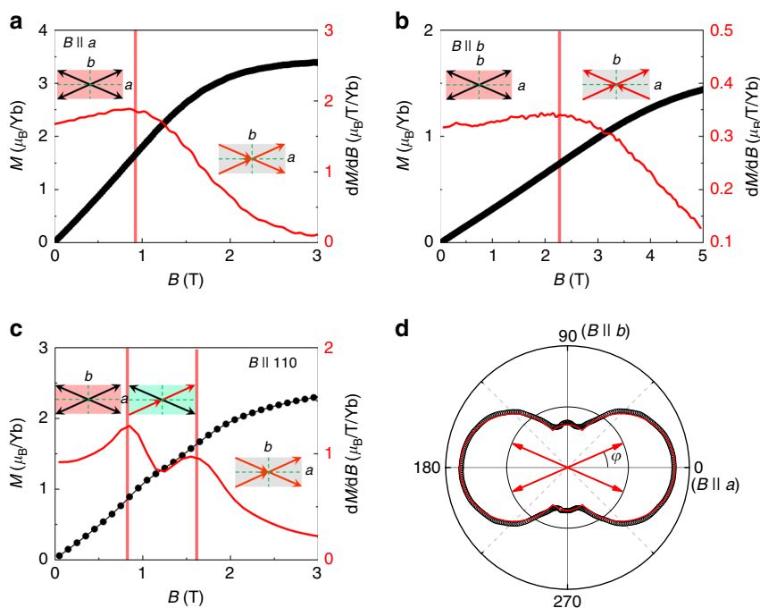
Fig. 1 Single-ion anisotropy of \text{YbAlO}_3 . a–c Field-dependent magnetization M (black circles) and magnetic susceptibility dM/dB (red line) of \text{YbAlO}_3 , measured at T = 2 K with field along the axes B \parallel a , B \parallel b and B \parallel [110] , as indicated. The insets are sketches of the magnetic moment configurations in different field ranges. d Angle-dependent magnetization measured at T = 2 K and B = 5 T. Red arrows schematically show a moment configuration of \text{Yb}^{3+} at zero field with angle \varphi = 23.5^\circ between the a -axis and the Yb magnetic moment. The solid line is the calculation, as described in the text
