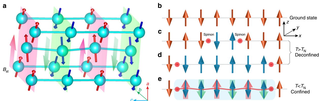
Fig. 2 Illustration of the magnetic structure and spinon confinement in \text{YbAlO}_3 . a Magnetic structure below T_N = 0.88 K, where the Yb Ising moments align antiferromagnetically (AFM) in chains along the c -axis. These one-dimensional (1D) chains are ferromagnetically (FM) coupled in ab -plane, which results in a net staggered field ( B_{st} ), as indicated by the large red and blue arrows. b–e Sketch of the spinon generation and confinement in a 1D AFM chain. Since only longitudinal fluctuations of \Delta S^z = 0 are observed in \text{YbAlO}_3 , even numbers of Yb moments are flipped in the AF ground state ( b ), creating pairs of spinons ( c ). These spinons can propagate freely (deconfined) along the chain at T > T_N ( c, d ), while in the presence of the effective staggered field at T < T_N , propagation of the spinons costs energy (confined) as the separation increases ( e )
