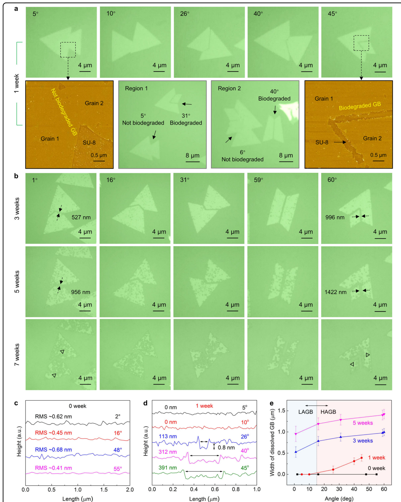
Fig. 2 Angle-dependent selective degradation of CVD-grown monolayer MoS 2 crystals in PBS solution. a OM and AFM images of the MoS 2 crystals with different misorientation angles (from 5° to 45°) after the crystals were kept in PBS solution (pH 7.4, 75 °C) for 1 week. b OM images of the MoS 2 crystals with different misorientation angles (from 1° to 60°) after the crystals were kept in PBS solution (pH 7.4, 75 °C) for 2–7 weeks. c, d AFM height profiles across the MoS 2 GB regions before and after degradation for 1 week. e The width of dissolved MoS 2 GB regions determined by both misorientation angles (from 1° to 60°) and degradation time (0–5 weeks)
