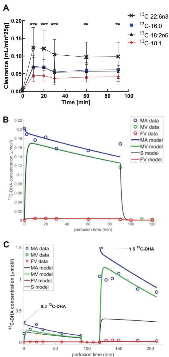
Fig. 1 Clearance of ^{13}\text{C} -labeled FFA and model prediction fitting the perfusion data for the ^{13}\text{C} -DHA placental transfer. (A) Clearance of ^{13}\text{C} -labeled palmitic acid (16:0), oleic acid (18:1), linoleic acid (18:2n6), and docosahexaenoic acid (22:6n3) was examined by placental perfusion ( n = 13 ). Kinetic of FFA transfer was investigated utilizing a closed (recirculated) maternal and open (nonrecirculating) fetal circulation. Mean ( \pm SD) ^{13}\text{C} -FFA clearance was calculated at time points 0, 10, 20, 30, 60, and 90 min. Two-way ANOVA and Bonferroni post hoc test were performed, ** p < 0.01 and *** p < 0.001 indicate significant differences between ^{13}\text{C} -DHA and other ^{13}\text{C} -FFA. (B) Circles represent the experimental data, solid lines represent the model predictions for the ^{13}\text{C} -DHA concentration of one lean subject. Blue represents the maternal artery (MA); green represents the maternal vein (MV); black represents the syncytiotrophoblast compartment (S); red represents the fetal vein (FV). Note that maternal vein concentrations were measured only at t = 90 min, whilst no experimental data were available for the tissue concentrations. Model parameter from one representative experiment is illustrated. (C) Model prediction when 0.3 \mu\text{mol/L} ^{13}\text{C} -DHA was added at time zero, followed by 1.5 \mu\text{mol/L} at t = 120 min. The total perfusion time was 210 min. Circles represent the experimental data, solid lines for the model predictions. Blue represents the maternal artery (MA); green represents the maternal vein (MV, t = 90 min only); black represents the syncytiotrophoblast compartment (S, no experimental data available); red represents the fetal vein (FV). The model parameters were estimated solely based on the data from the first phase of the perfusion experiment (0–120 min) and then applied to predict the second phase of the experiment (120–210 min). Note that the initial concentration values used for the model were based on the initial dose administered. This particular experiment was performed once.
