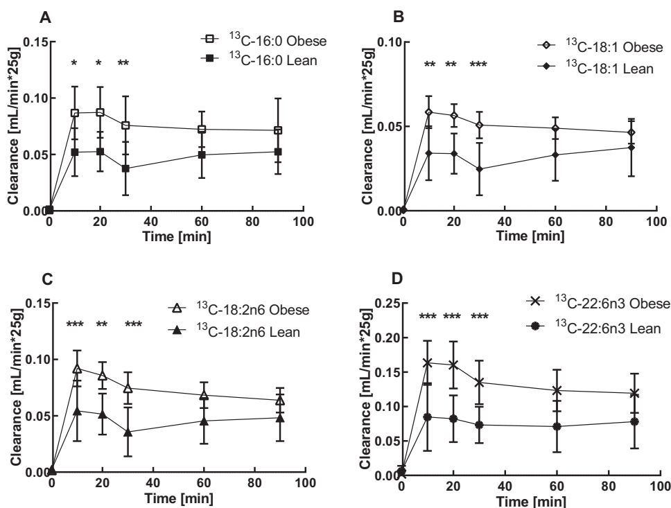
Fig. 2 Clearance of ^{13}\text{C} -labeled FFA in placentae of lean versus obese women.
