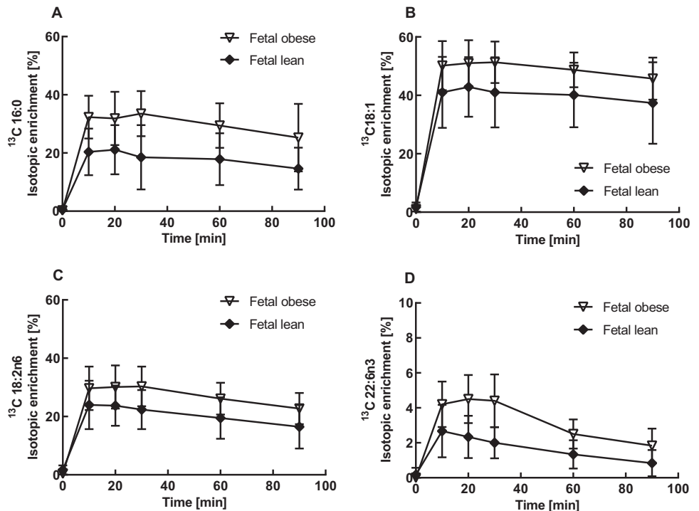
Fig. 3 Isotopic enrichment in fetal effluents. ^{13}\text{C} -labeled and endogenous FFA were determined in fetal venous samples A palmitic acid (16:0), B oleic acid (18:1), C linoleic acid (18:2n6), and D docosahexaenoic acid (22:6n3). Mean ( \pm SD) ^{13}\text{C} -isotopic enrichment in perfusion experiments, lean ( n = 8 ) and obese ( n = 7 ) placentae were calculated at time points 0, 10, 20, 30, 60, and 90 min and is expressed as percentage.
