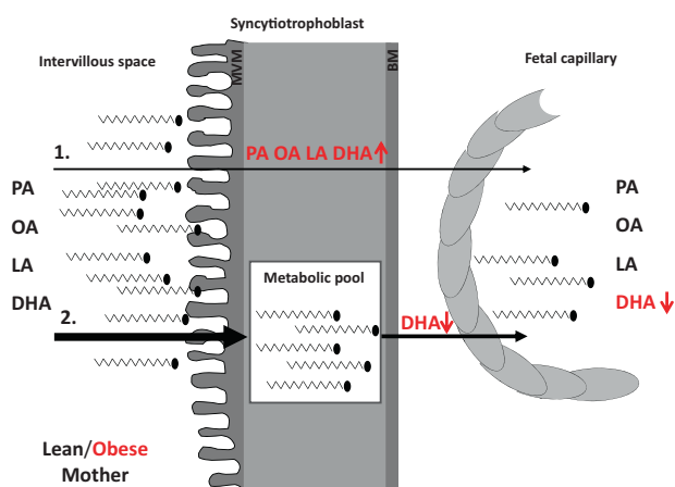
Fig. 4 Model for FFA transfer across the placental barrier. (1) FFA derived from maternal plasma is transferred directly across the placental syncytiotrophoblast to the placental–fetal endothelium. In placentae of obese women transfer rates for all examined FFA are elevated (red arrow). (2) Simultaneously, maternal FFA are taken up by the placenta and mass balance calculations suggest an enrichment of FFA within the tissue (metabolic pool). Out of the metabolic pool, FFA may be released to the fetal circulation. In fact, mobilization of DHA was reduced in placentae of obese women, resulting in lower DHA levels in the fetal capillaries/circulation. MVM microvillous membrane, BM basal membrane, PA palmitic acid, DHA docosahexaenoic acid, LA linoleic acid, and OA oleic acid.
