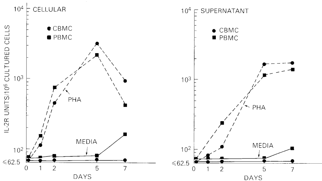
Fig. 1. Time course of cellular and supernatant IL-2R production by PHA-activated CBMC and adult PBMC in vitro . CBMC (●) and PBMC (■) were cultured with media alone (—) or PHA (---) for various time periods in vitro . Detergent-solubilized cells ( left ) and cell-free culture supernatants ( right ) were analyzed for IL-2R by enzyme-linked immunosorbent assay (see "Materials and methods").
